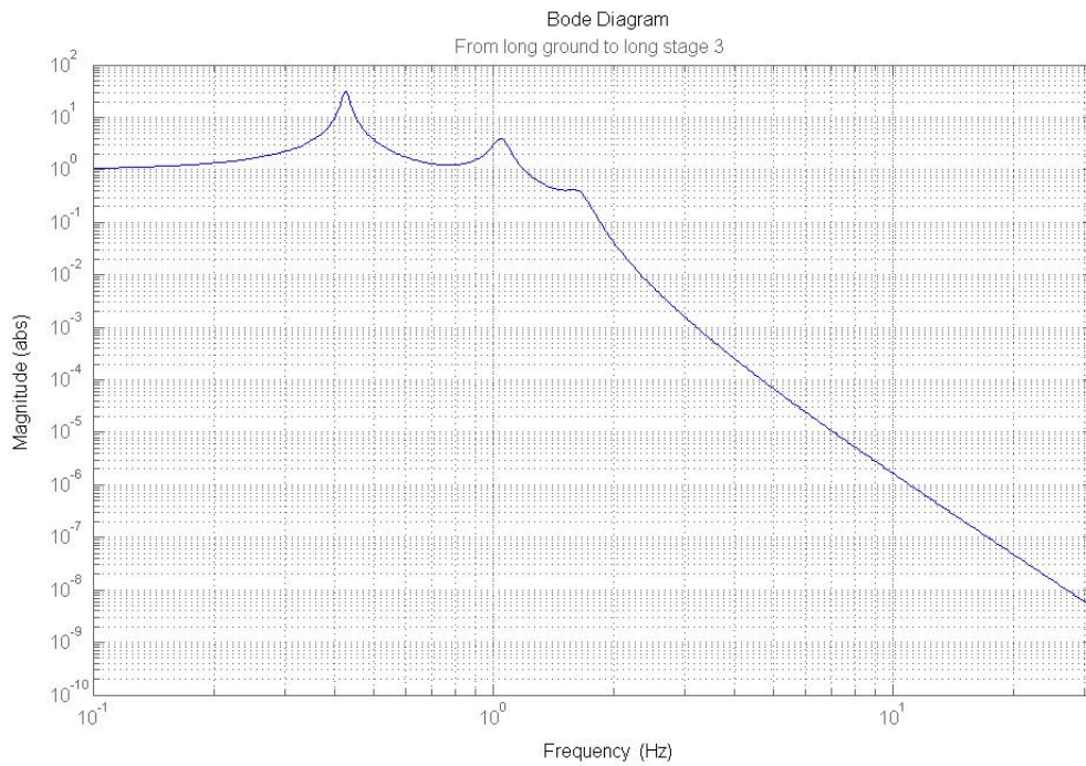
Figure 5. Vertical transfer function for beamsplitter triple suspension (with eddy current damping).
