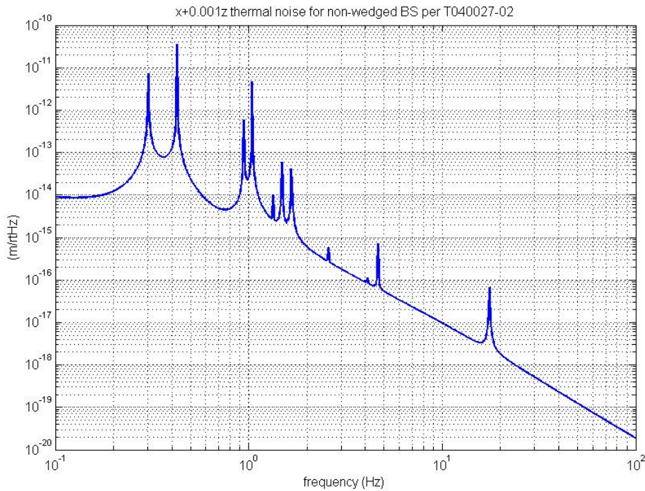
Figure 2. Thermal noise for BS on steel wires (unwedged case) with longitudinal and 0.001 times vertical summed quadratically. The noise is dominated by the longitudinal contribution except at the vertical mode peaks including the highest vertical mode at 17.5 Hz. The level at 10 Hz is 10^{-17} m/rt Hz, below the requirement of 2 \times 10^{-17} m/rt Hz.
