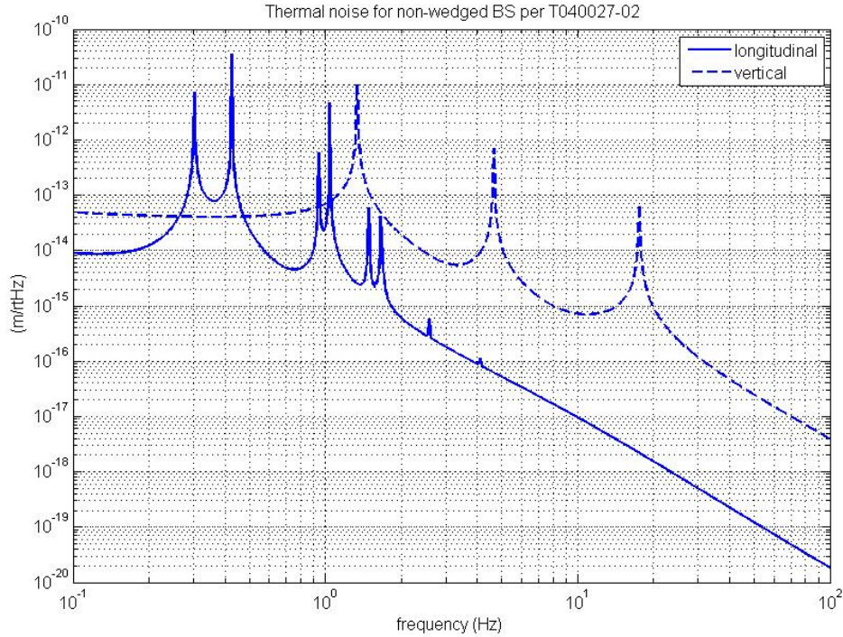
Figure 1. Thermal noise for BS on steel wires, parameters as referenced in Appendix B (unwedged case). Longitudinal and vertical noise estimates are shown separately. Note that at frequencies above the highest vertical mode at 17.5 Hz the vertical thermal noise curve lies more than a factor of 100 above the longitudinal curve.
