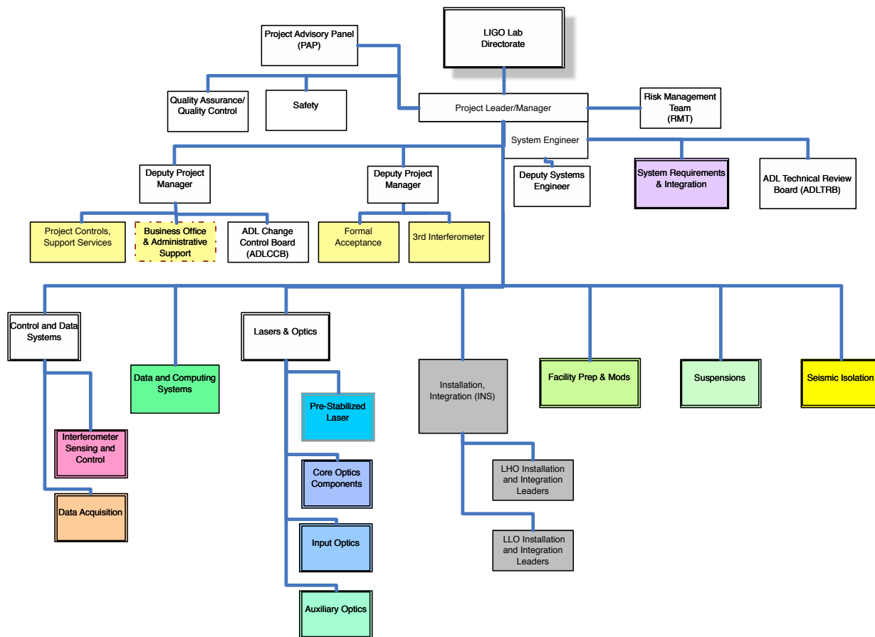
Advanced LIGO Project Organization 2013-10-04 LIGO-T1200224-v3
