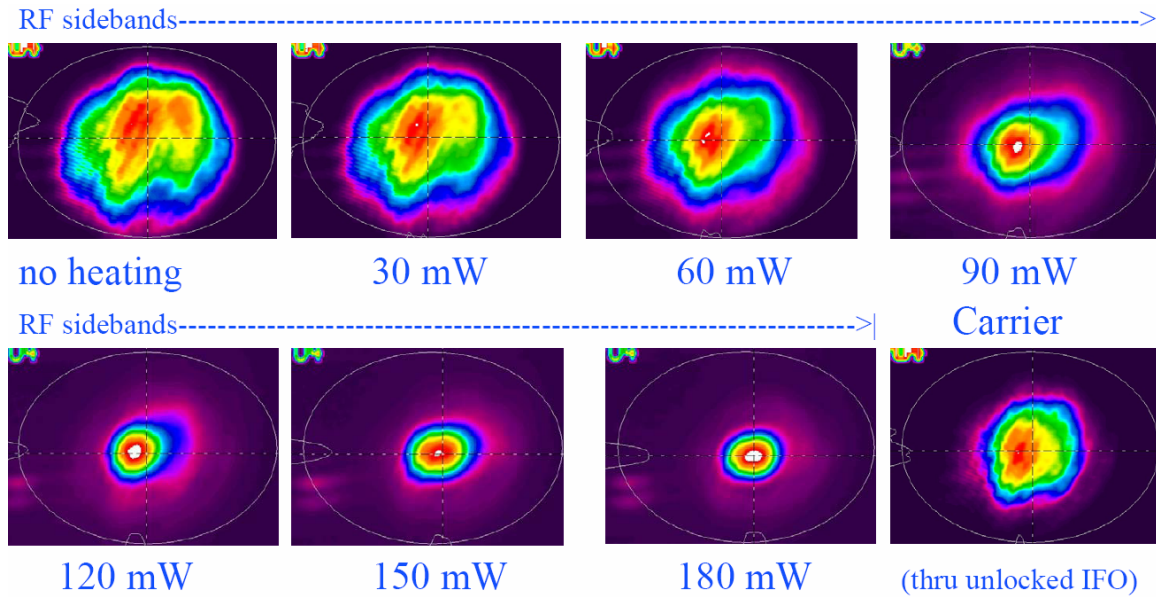
Figure 16 RF sideband mode shape control using thermal compensation. Note the optimum overlap between RF sideband and carrier mode at 90 mW heating power.
