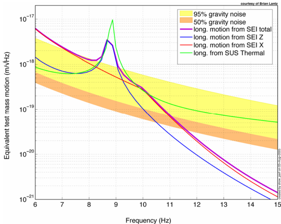
Figure 2 Predicted test mass displacement noise. The orange and yellow shaded regions are the expected longitudinal (beam direction) motion from direct gravity coupling, at 50 th and 95 th percentile ground motion measured at the LIGO sites; this dominates over the seismic noise above 11 Hz or so. The red, blue and purple lines are, respectively, the contributions to test mass motion from horizontal and vertical seismic isolation system motion and the total seismic contribution at about the 90 th percentile level. The green curve is the expected suspension (pendulum) thermal noise; it exceeds the seismic noise above about 10.3 Hz.
