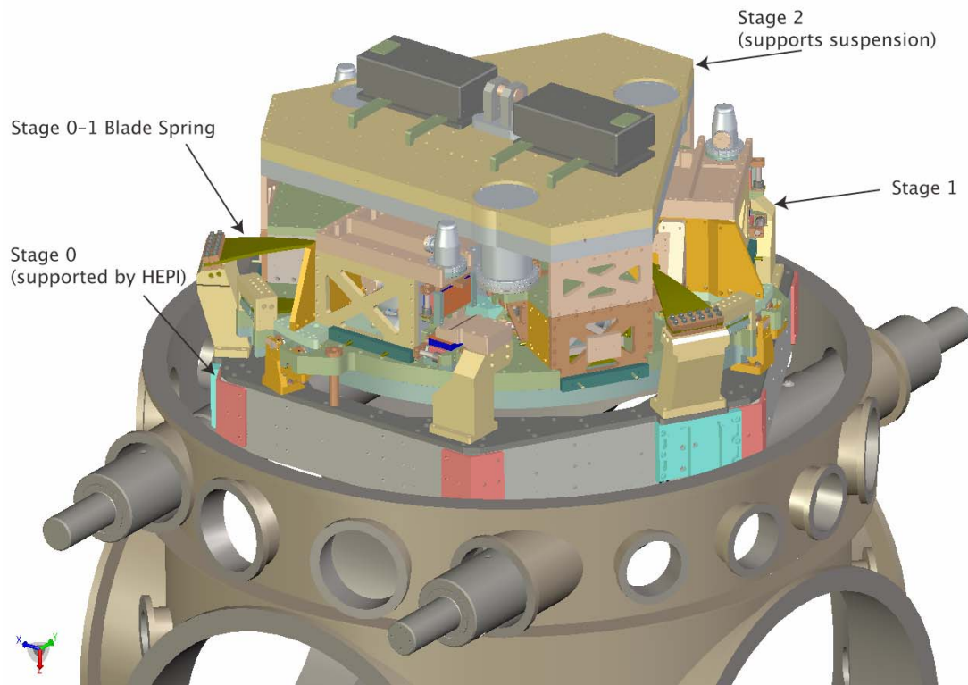
Figure 3 Computer rendering of the prototype two-stage in-vacuum active seismic isolation system (ISI) for the test-mass (BSC) vacuum chambers, which is under construction as of this writing. The outside frame (stage 0) supports the stage 1 from three trapezoidal blade springs and vertical flexure rods. Stage 2, which supports the payload, is likewise suspended from stage 1. The bottom of stage 2 is an optics table under which the test mass suspensions are mounted.
