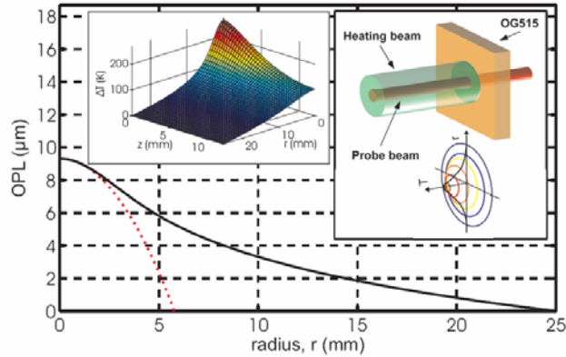
Figure 13 Calculated radial dependence of the optical path difference (OPD) assuming 4 W of heating power in a 7.2 mm diameter beam. The solid line results from an exact solution of the thermal diffusion equation; the dotted line displays the OPD assuming a parabolic lens. Right inset: schematic view of laser adaptive mode control. Left inset: the spatial dependence of the temperature profile \Delta T(r,z) .
