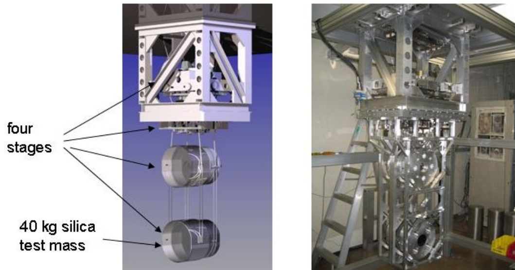
Figure 5 Left: schematic diagram of quadruple suspension showing main chain and parallel reaction chain for interferometer control actuation, with lower support structure removed for clarity. Right: all-metal controls prototype under test at Caltech
