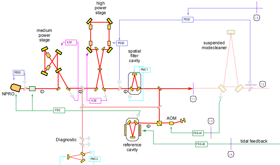
Figure 9 Schematic of the Advanced LIGO PSL.
