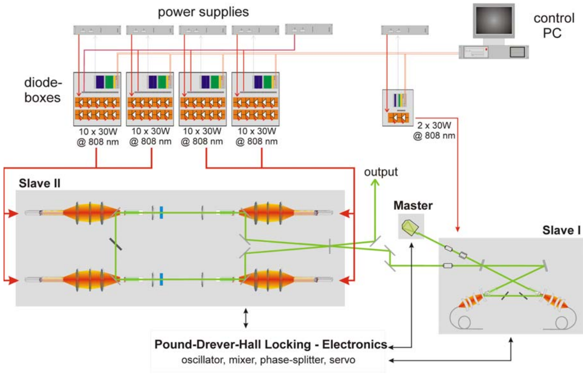
Figure 8 Schematic of the Advanced LIGO laser showing the single-frequency master laser, an injection-locked medium power stage (labeled Slave I) followed by the high power stage (labeled Slave II)
