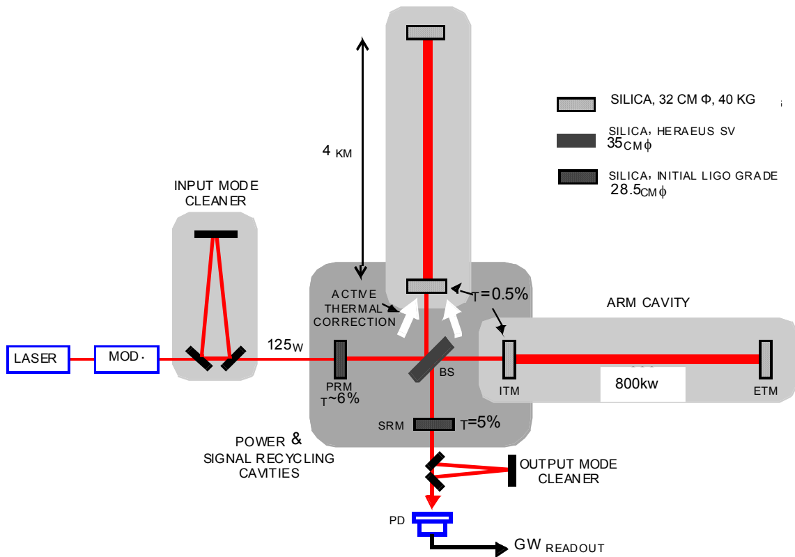
Figure 1 Schematic of an Advanced LIGO interferometer, with representative mirror reflectivities optimized for neutron star binary inspiral detection. Several new features compared to initial LIGO are shown: more massive test masses; 20x higher input laser power; signal recycling; active correction of thermal lensing; an output mode cleaner. (ETM = end test mass; ITM = input test mass; PRM = power recycling mirror; SRM = signal recycling mirror; BS = 50/50 beam splitter; PD = photodetector; MOD = phase modulation). Seismic Isolation system, Optics Suspensions, and the mode-matching and beam-coupling telescopes not shown.
