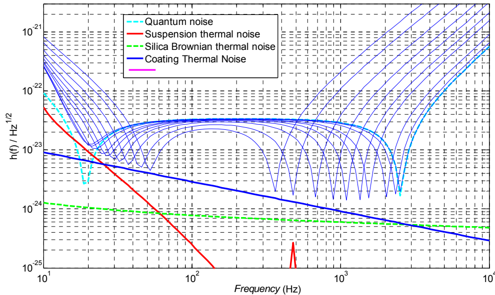
Figure 17 Strain sensitivity curves for a narrowband interferometer. By changing from a signal recycling mirror optimized for broadband operation to one chosen to give optimum performance around 800 Hz, good performance at a selected frequency between \sim 400 – 2000 Hz can be achieved by tuning the signal mirror position microscopically; the set of curves shown span a mirror motion of less than a micron. At the lower end of the range, coating thermal noise limits the performance; at higher frequencies, above \sim 500 Hz, the quantum noise limits the best performance (modeled using Bench 23 )
