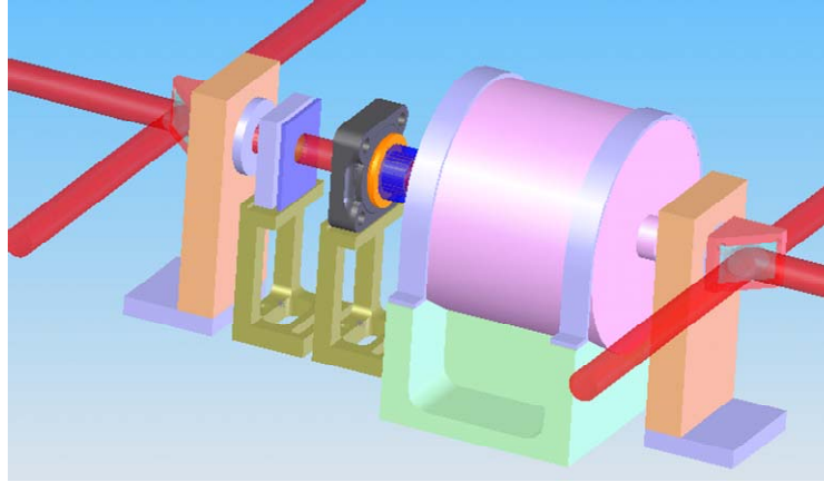
Figure 12 Schematic drawing of the FI, showing from right (beam entrance) to left i) initial polarizer, ii) Faraday rotator, iii) 1/2 waveplate, iv) thermal lens compensator, and v) final polarizer.
