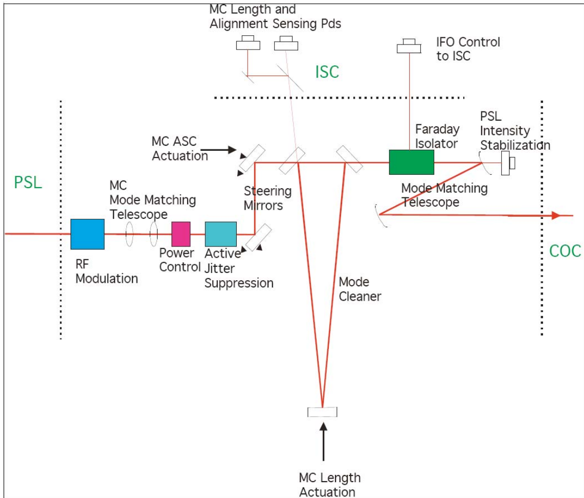
Figure 10 Schematic diagram of the Advanced LIGO Input Optics (IO) subsystem.
