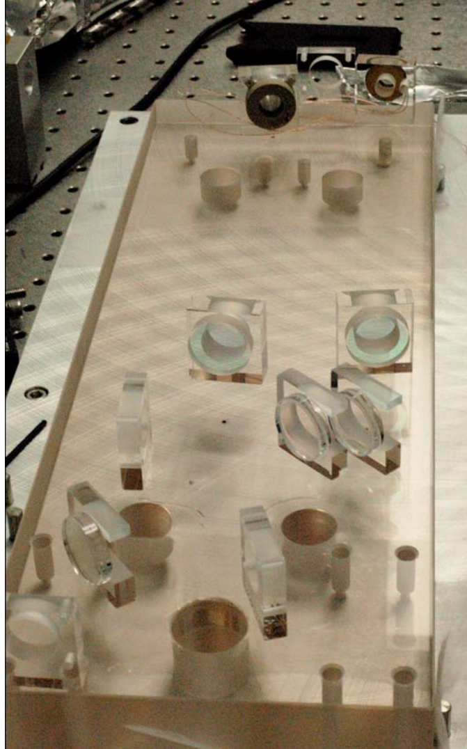
Figure 17: The Output Mode Cleaner for the enhancements to initial LIGO; a prototype for Advanced LIGO.
