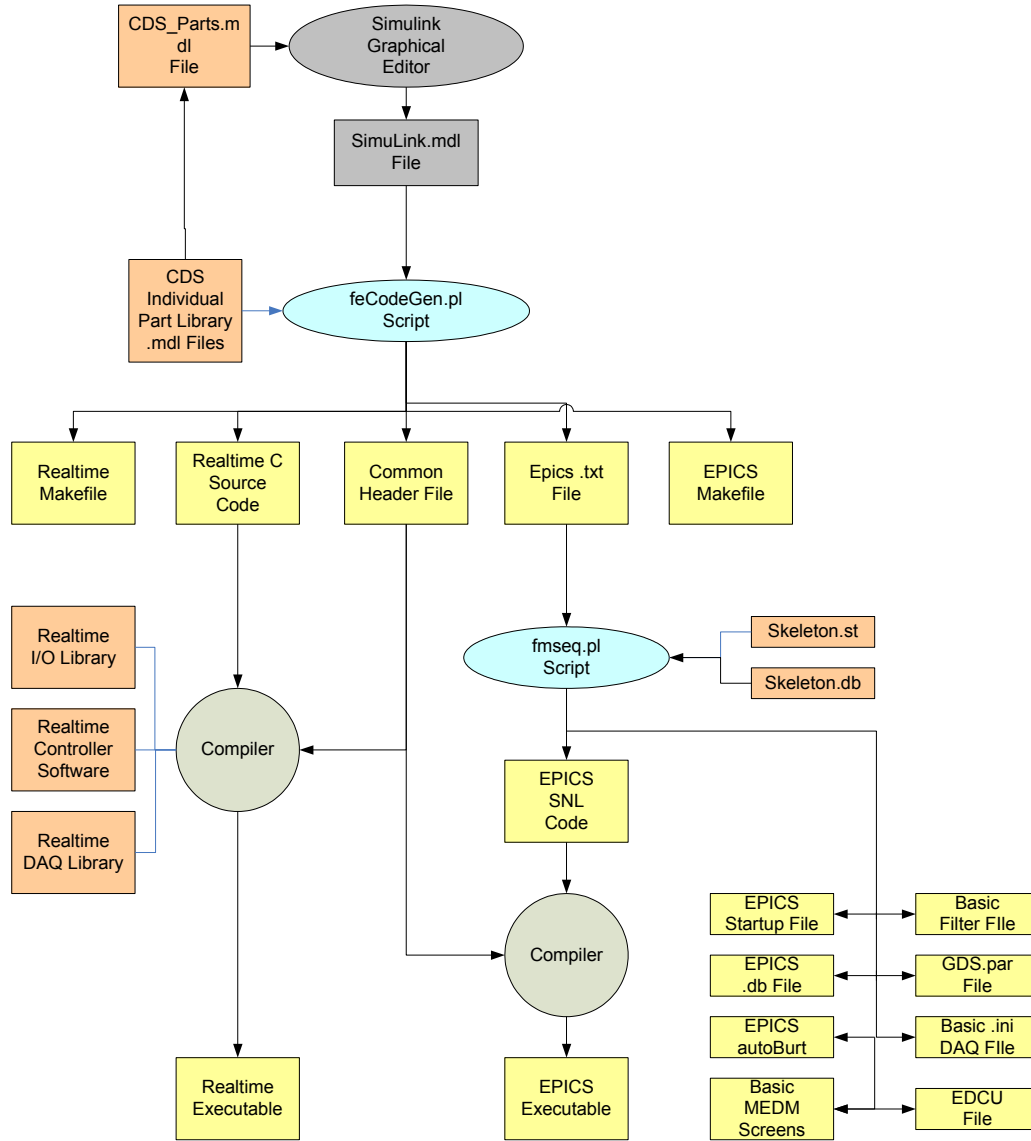
Figure 4: Code Generation
