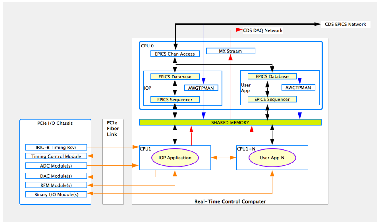
Figure 5: Run-time Software Overview
