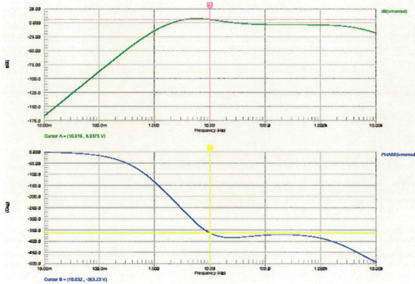
Figure 4: Top Driver Response at Monitor Output
