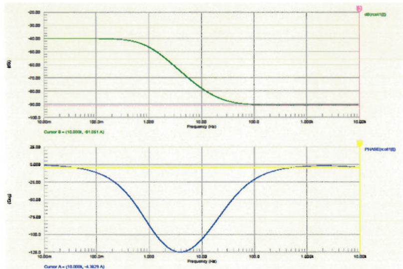
Figure 2: Top Driver Response (Run Mode)
