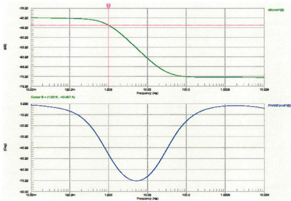
Figure 1: Top Driver Response (Acquire Mode)
