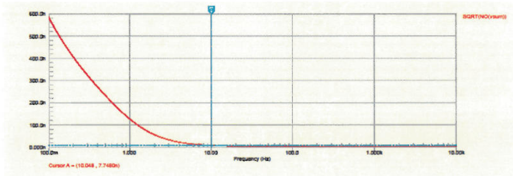
Figure 3: Top Driver Output Noise
