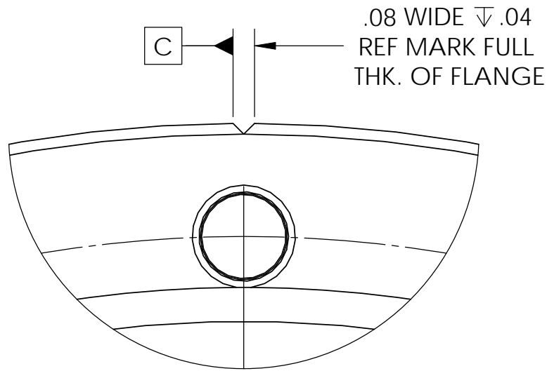
DETAIL E SCALE 2 : 1
