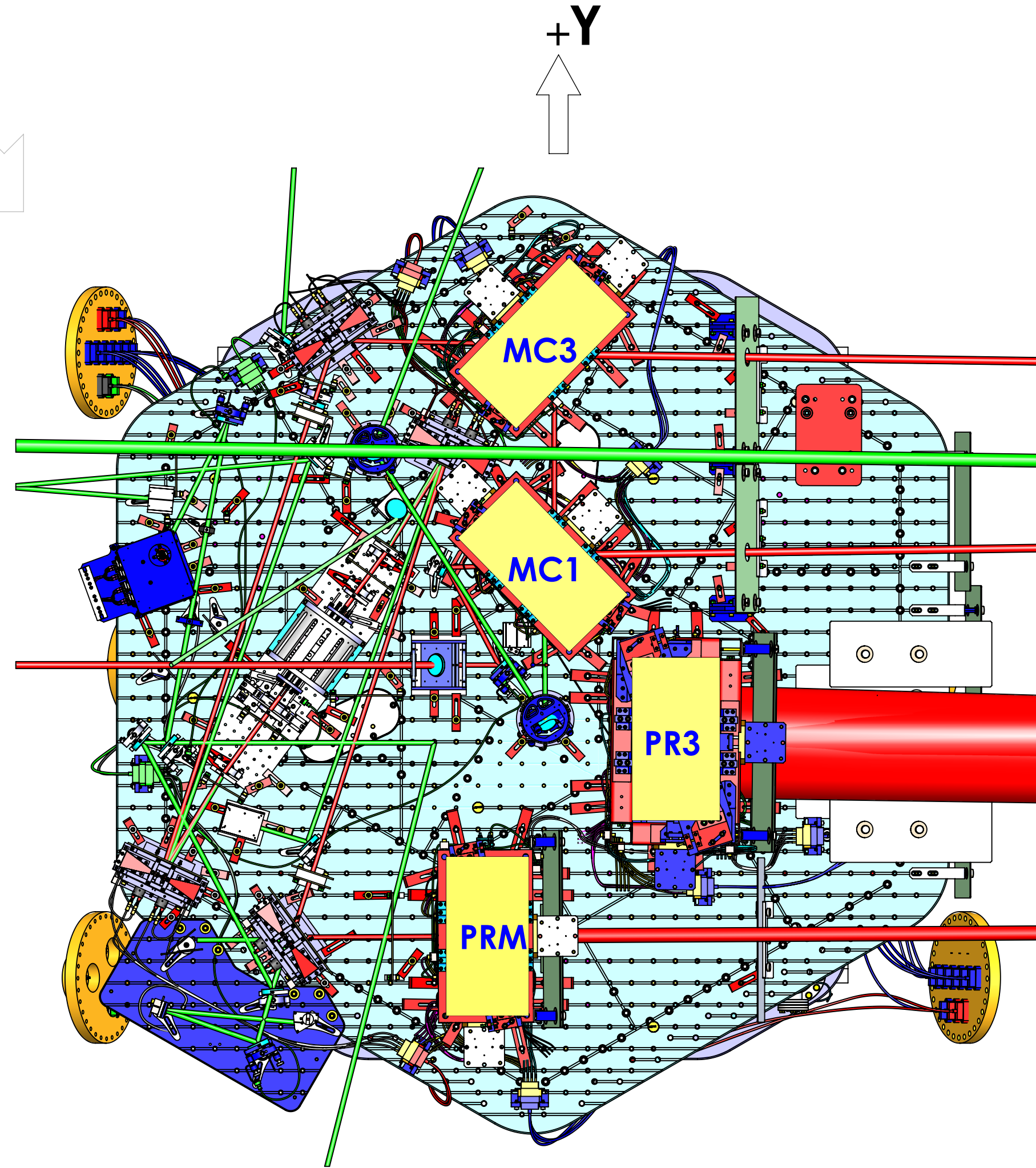
TOP VIEW
