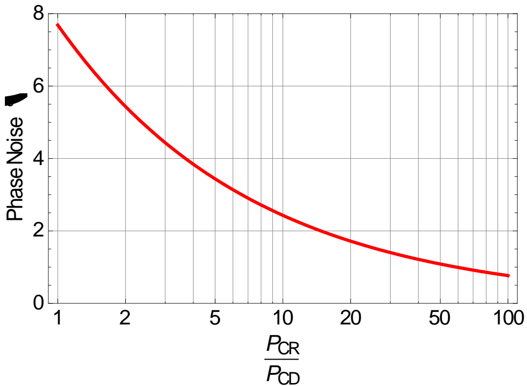
Figure 4: Phase noise due to the RF sidebands at the AS port after the OMC. The curve is given as a function of the ratio of the total carrier power over the carrier power due to contrast defect.
