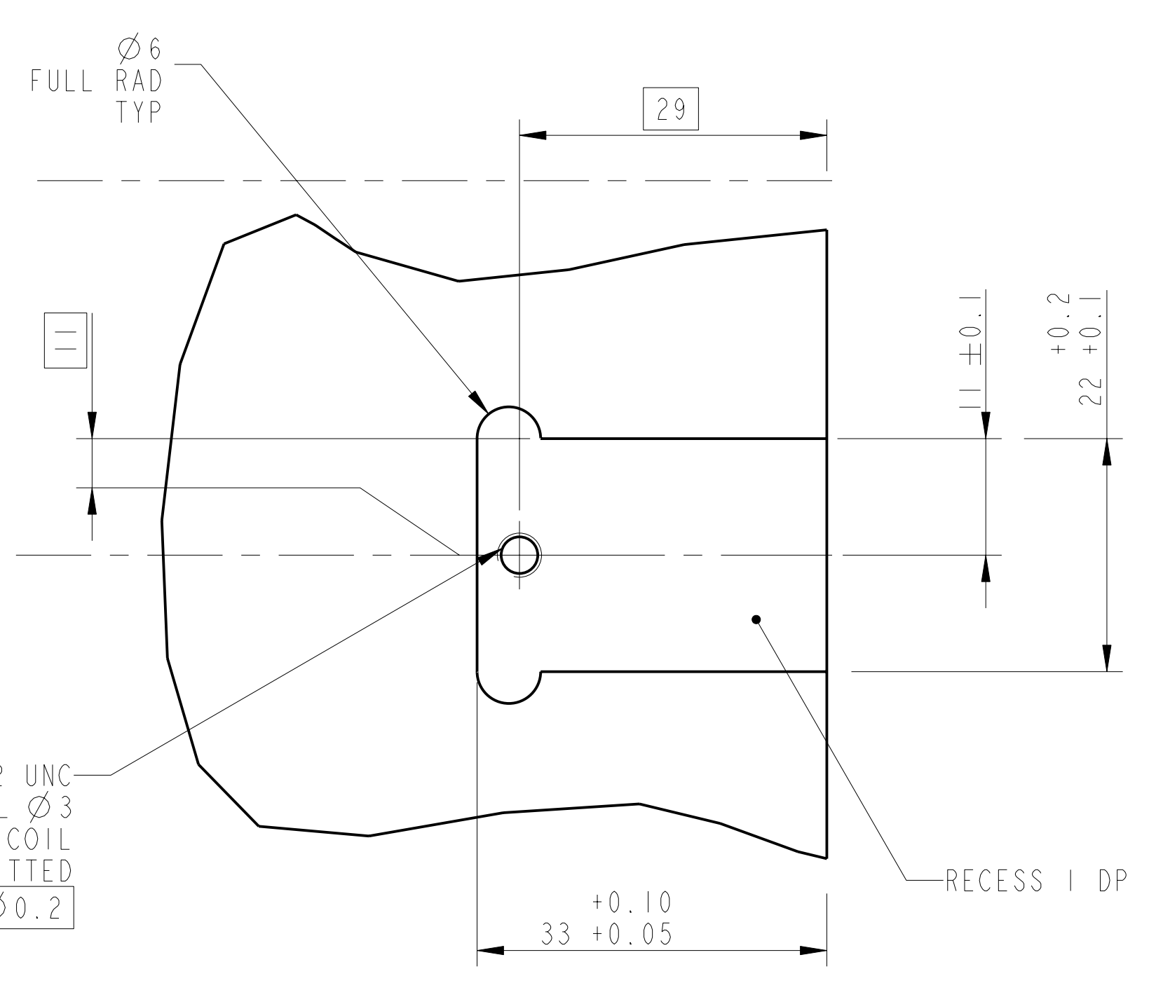
DETAIL B SCALE 2:1 2 POSITIONS
