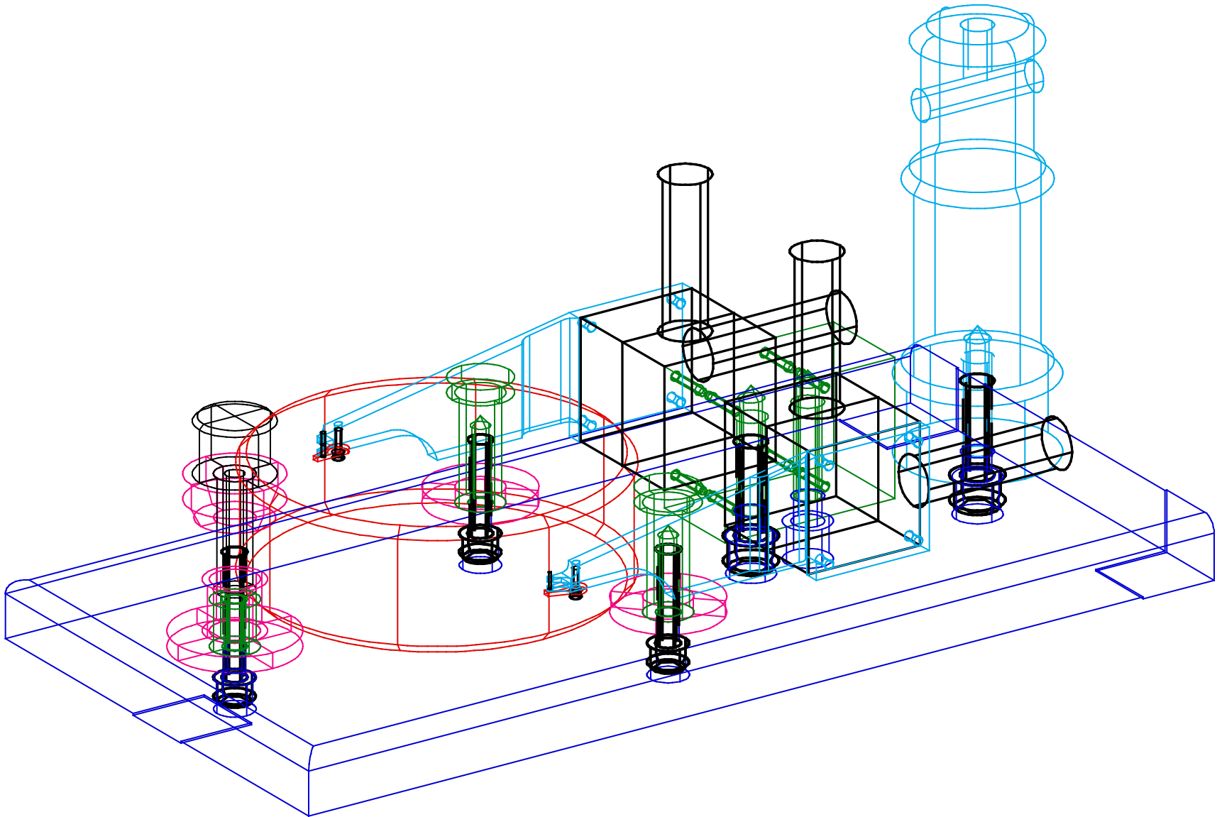
D000335-v2 Small Optics Guide Rod Gluing Fixture Assembly (SOGF) 1-12-2001
