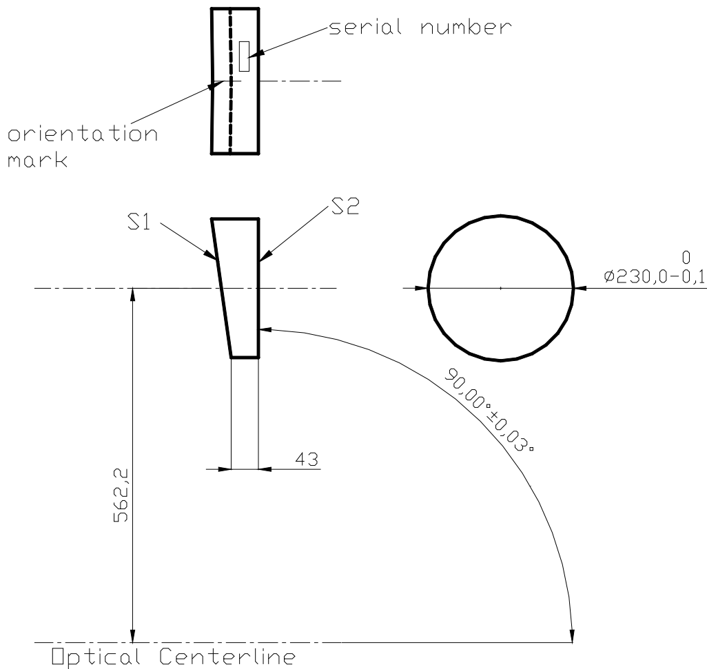
Figure 1: Mirror drawing, parabolic primary mirror
