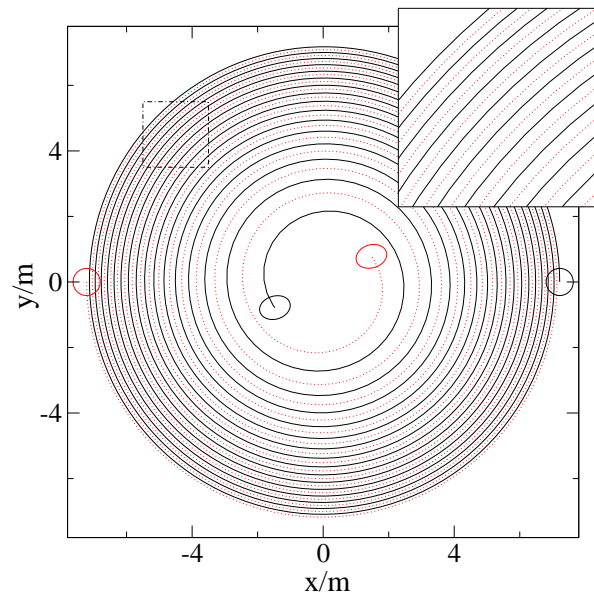
FIG. 3: Coordinate trajectories of the centers of the black holes. The small circles/ellipsoids show the apparent horizons at the initial time and at the time when the simulation ends and wave escorting begins. The inset shows an enlargement of the dashed box.
