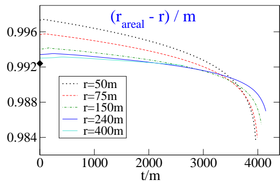
FIG. 9: Difference between areal radius r_{\text{areal}} and coordinate radius of select extraction surfaces. r_{\text{areal}} remains constant to within 0.01m during the evolution. The diamond indicates M_{\text{ADM}}/m of the initial data.
