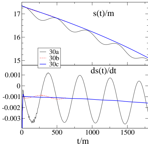
FIG. 1: Proper separation (top panel) and its time derivative (lower panel) versus time for short evolutions of the d = 30 initial data sets '30a', '30b', and '30c' (see Table I). These three data sets represent zero through two iterations of our eccentricity-reduction procedure. The orbital eccentricity is reduced significantly by each iteration.
