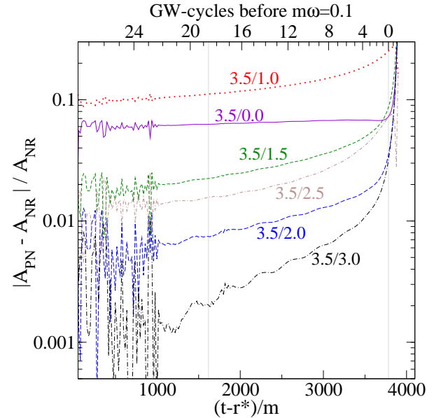
FIG. 20: TaylorT4 amplitude comparison for different PN orders. Shown is the relative difference in gravitational wave amplitude between TaylorT4 and numerical Y_{22} waveforms as a function of time. Matching is performed at m\omega_m = 0.04 (indicated by the left vertical grey line, whereas the right vertical grey line indicates m\omega = 0.1 ). All curves use 3.5PN order in phase but different PN orders (as labeled) in the amplitude expansion.
