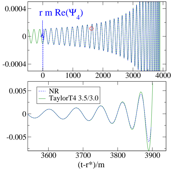
FIG. 19: Numerical and TaylorT4 3.5/3.0 waveforms. The PN waveform is matched to the numerical one at m\omega_m = 0.04 , indicated by the small circle. The lower panel shows a detailed view of the end of the waveform.
