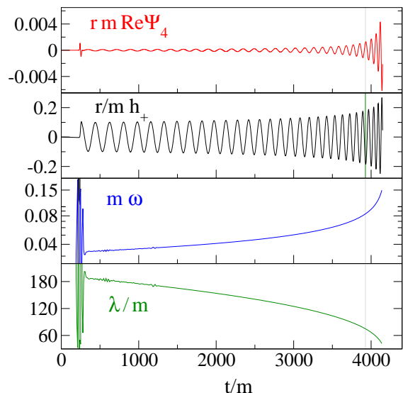
FIG. 5: Gravitational waveform extracted at r = 240m . From top panel to bottom: The real part of the l = 2, m = 2 component of r\Psi_4 ; the gravitational wave strain, obtained by two time integrals of \text{Re}(r\Psi_4) ; the frequency of the gravitational wave, Eq. (15); the gravitational wavelength, \lambda = 2\pi/\omega . The vertical grey line at t \approx 3930m indicates the time when ‘wave escorting’ starts.
