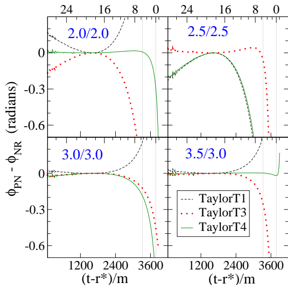
FIG. 21: Phase comparison for different PN approximants at different PN orders, matched at m\omega_m = 0.04 . Shown is the difference in gravitational wave phase between each post-Newtonian approximant and the numerical Y_{22} waveforms as a function of time. The two vertical grey lines indicate when the numerical simulation reaches m\omega = 0.063 and 0.1 , respectively; the labels along the top horizontal axes give the number of GW-cycles before m\omega = 0.1 .
