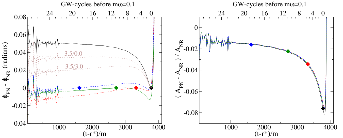
FIG. 18: Comparison of numerical simulation with TaylorT4 3.5/2.5 waveforms. Left: Difference in gravitational wave phase. Right: Relative amplitude difference. Plotted are comparisons for four values of \omega_m . The filled diamond on each curve shows the point at which \phi = \omega_m . The left plot also includes two phase comparisons with expansions of different PN order in amplitude, as labeled.
