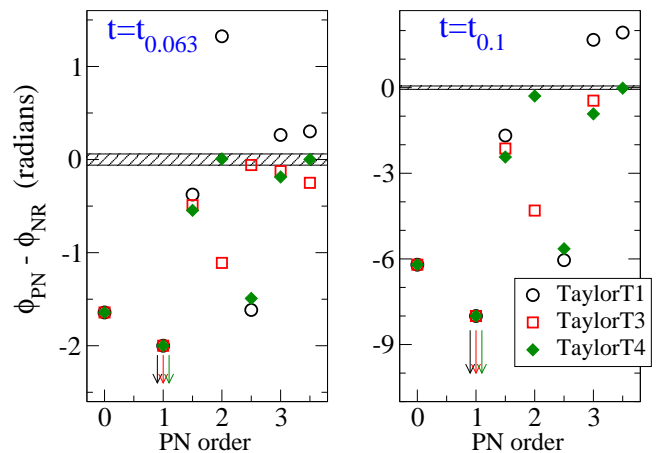
FIG. 22: Phase differences between numerical and post-Newtonian waveforms at two selected times close to merger. Waveforms are matched at m\omega_m = 0.04 , and phase differences are computed at the time when the numerical simulation reaches m\omega = 0.063 (left panel) and m\omega = 0.1 (right panel). Differences are plotted versus PN order (equal order in phase and amplitude, except the '3.5 PN' points are 3.5/3.0). The 1PN data points are off scale, clustering at -5.5 radians (left panel) and -15 radians (right panel). The thin black bands indicate upper bounds on the uncertainty of the comparison as discussed in Sec. V A.
