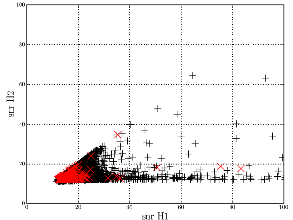
FIG. 7: Scatter plot of SNR for coincident triggers in H1-H2 times. The light colored crosses represent in-time coincident triggers and the black pluses represent time-shift coincident triggers that we use to estimate the background. Note that due to our signal based veto on H1/H2 SNR we see no coincident triggers with \rho_{H1} < \rho_{H2} .
