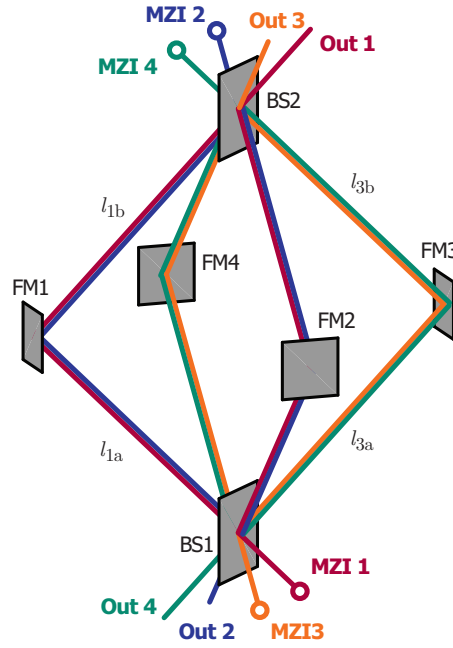
Figure 1. The schematic of three dimensional DFI. The laser light propagates on the ridge line of the octahedron to form four simple Mach-Zhender interferometers. There are two beam splitters (BS) and four folding mirrors (FM) at the spatially symmetric apexes of the octahedron.
