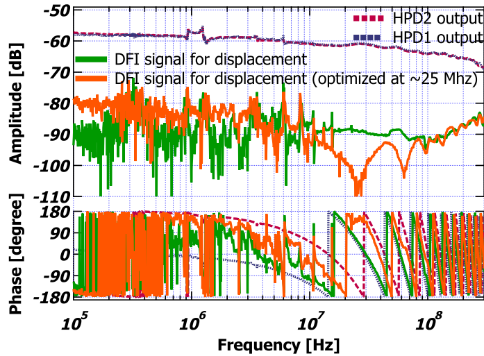
Figure 3. The transfer function from the displacement simulator to the interferometer output. The displacement information on the HPD1 and HPD2 is significantly cancelled in the DFI signals.
