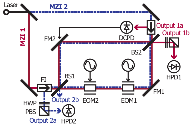
Figure 2. Practical setup for the partial demonstration of DFI. This is one pair of bidirectional MZIs, which is a part of 3D DFI, to confirm the cancellation of folding mirrors and the finite response to the GW signals.
