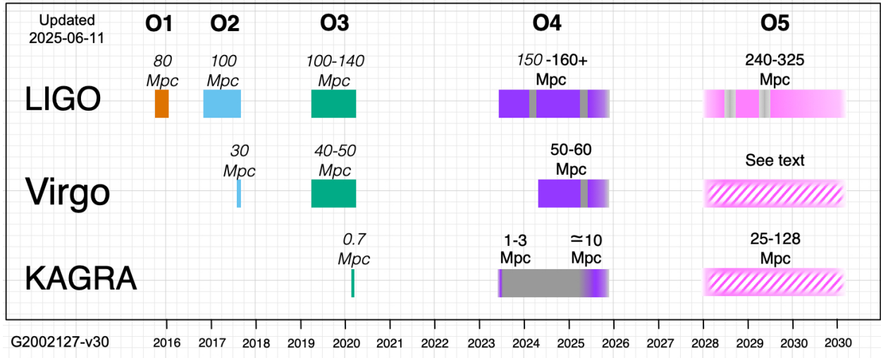
Figure 2: Timeline of past and future observing runs, current at the time of writing. The expected schedule and sensitivity may evolve with time. Gray shading indicates commissioning times. Currently, the Virgo Collaboration is reassessing its plans for O5 and both the entry date into O5 and the target sensitivity are unclear. See https://observing.docs.ligo.org/plan for the most up-to-date observing plans. Figure adopted from https://dcc.ligo.org/G2002127/public/ .
