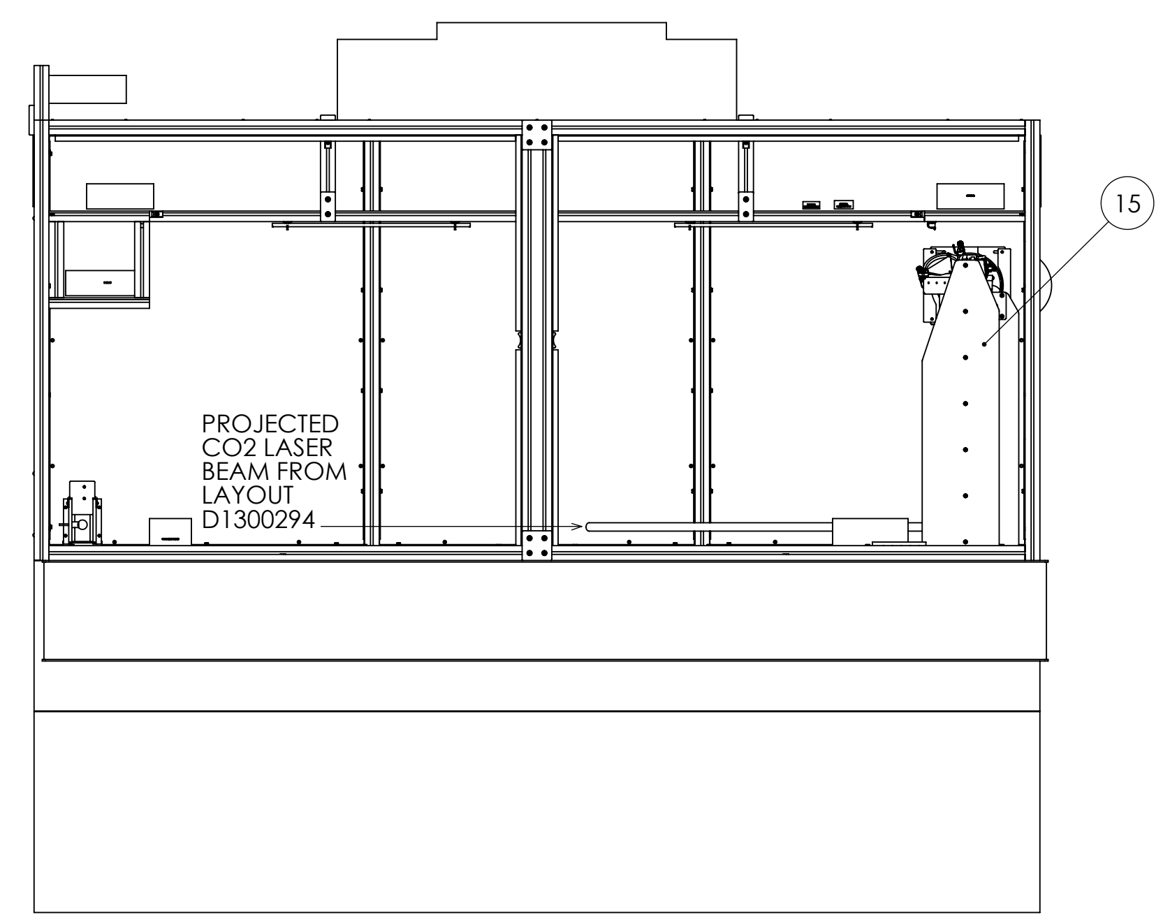
FACING TWO HINGED DOORS OF THE TABLE (DOORS OMITTED FOR CLARITY)
