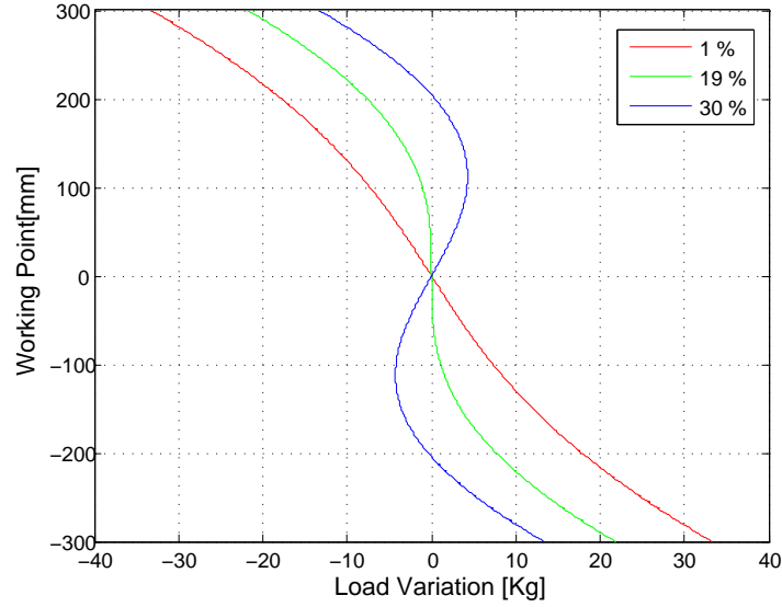
Figure 2.8: Equilibrium Point displacement for a variation of the payload's mass in correspondence of several compressions. The compression ratio is defined as (l_{0x} - x_0)/(l_{0x}) .
