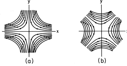
Figure 1.1: Direction of space deformation for a gravitational wave propagating along the z -axis, + polarization (a) and \times polarization (b)
