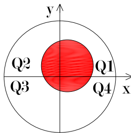
Figure 4.13: QPD sensor. The signal from each quadrant is proportional to the area covered by the beam spot (red). The coordinates of the beam spot's center are given by the differences between the output signals.
