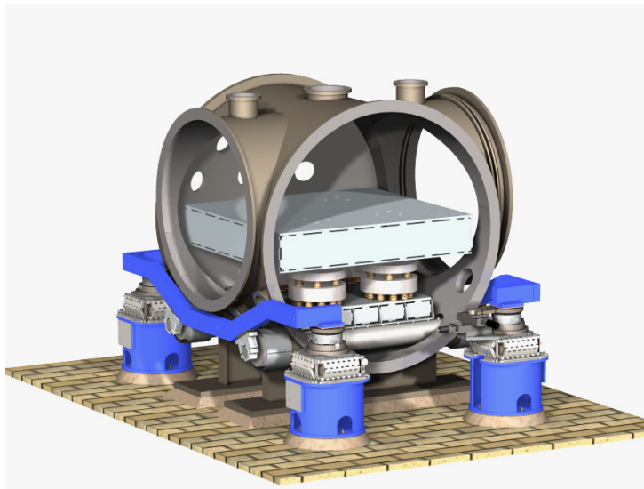
Figure 2.2: LIGO I chamber and seismic attenuation stacks.
