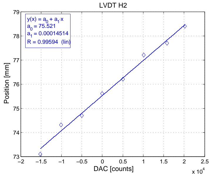
Figure 4.8: H2 LVDT calibration results. The fit gives a coefficient of 0.18 \mu\text{m}/\text{count}
