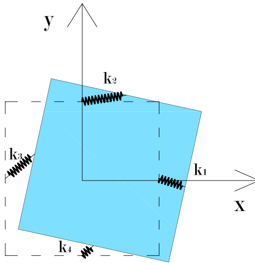
Figure 2.20: Dynamical model for the horizontal degrees of freedom
