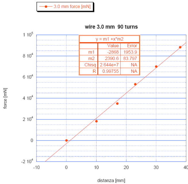
Figure 3.5: 3 mm wire spring stiffness measurement
