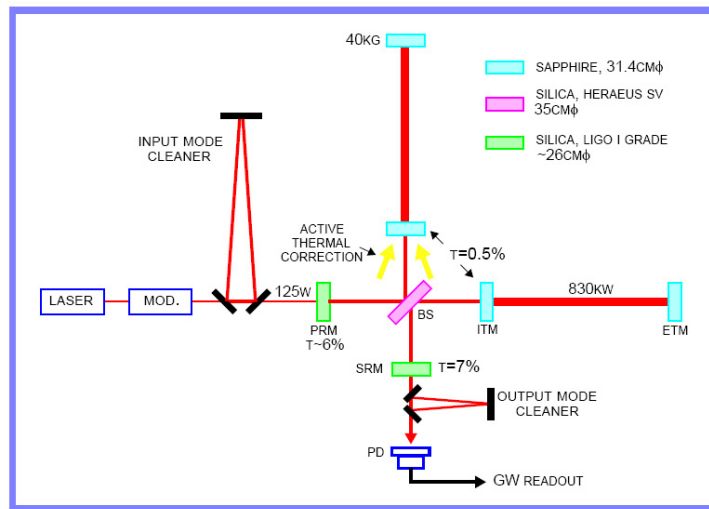
Figure 2.1: Basic layout of an advanced LIGO interferometer.
