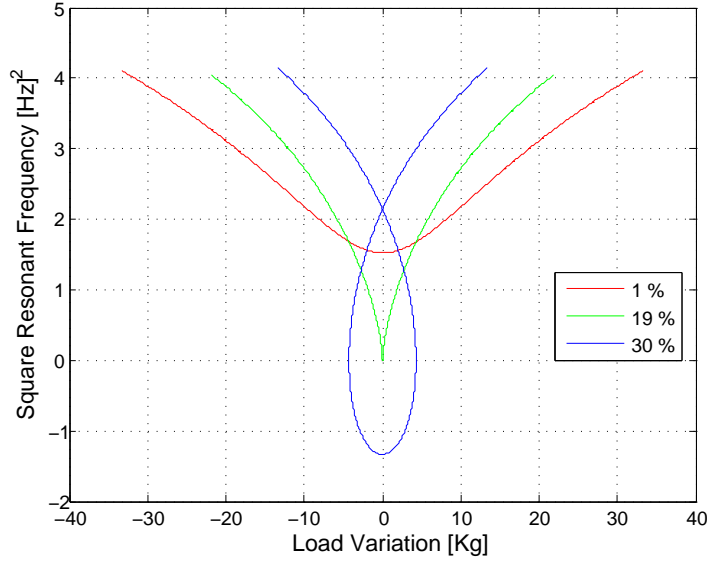
Figure 2.9: Dependence of the squared resonant frequency to the variation of the payload's mass at the equilibrium point.
