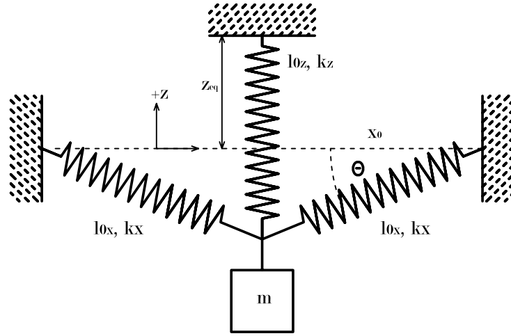
Figure 2.7: GAS Springs Model
