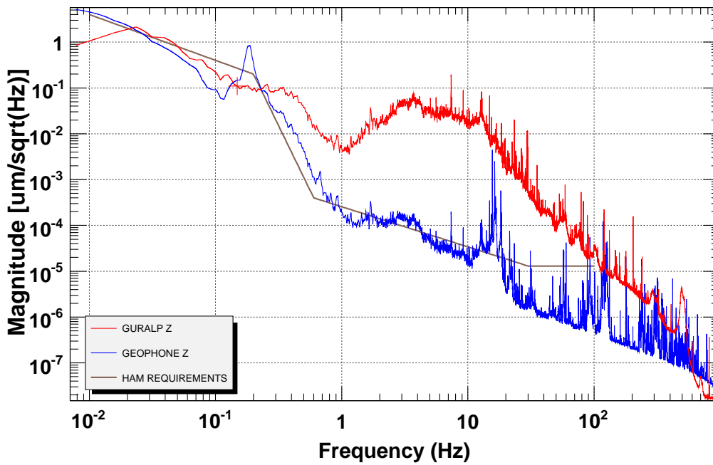
Figure 6.9: The plot shows the power spectrum on the x direction (upper plot) and of the vertical direction z (lower plot) each one compared with the reference given by the correspondent displacement spectra from the seismometers on the ground (red curves) and the HAM requirements. DC, damping and Resonance Gain controls are active.
