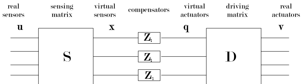
Figure 5.2: Diagonalization scheme
