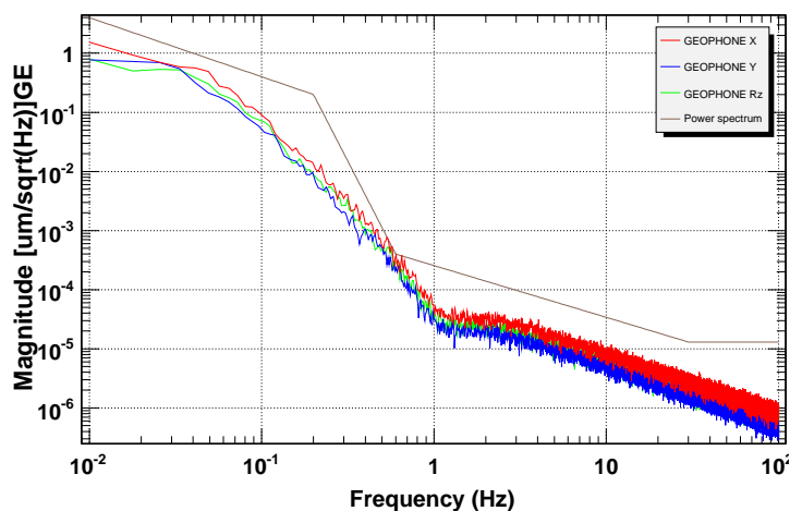
Figure 6.8: Geophones noise floor measured disconnecting the sensors from the readout board.
