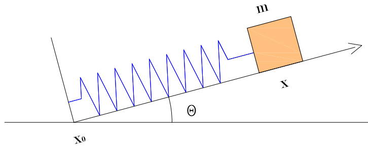
Figure 4.12: Model to explain the tilt to horizontal coupling in the horizontal geophones on the optics table.
