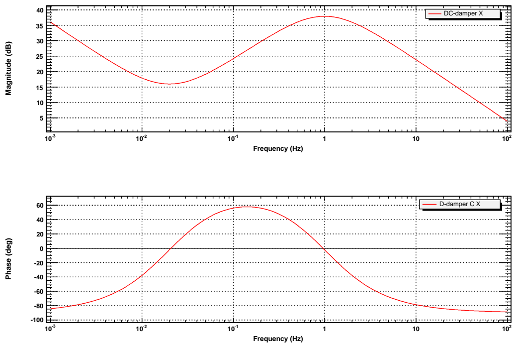
Figure 6.10: The plot shows the transfer function amplitude and phase of the position and damping combined control for the horizontal mode X that we applied to obtain the performances which met the seismic attenuation requirements. The same filter shape, but with different gains and locations of poles and zeros adapted to the specific physical plant responses are applied to the other modes.
