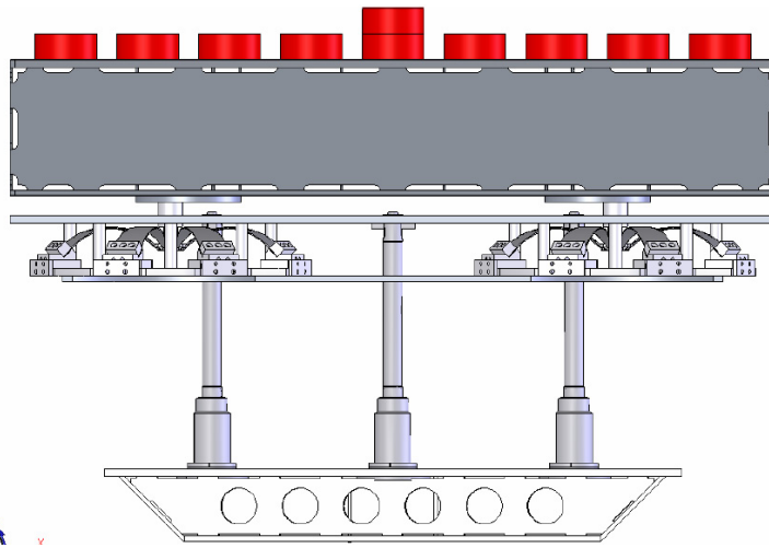
Figure 2.3: HAM-SAS Assembly
