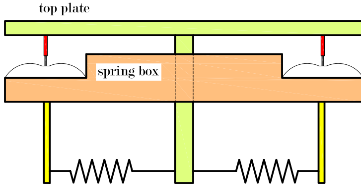
Figure 2.14: Scheme of the tilt correcting springs added between the top plate and the spring box.
