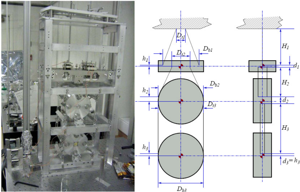
Figure 4.2: Triple pendulum and sketch of a representing model. The triple pendulum is the last stage of the seismic isolation. Its role is to filter the high ( >10\text{Hz} ) frequencies noise using three stages of passive isolation in the horizontal directions and two stages of isolation in the vertical one [43].
