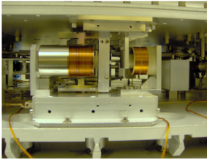
Figure 2.21: Horizontal coil actuator and LVDT.
