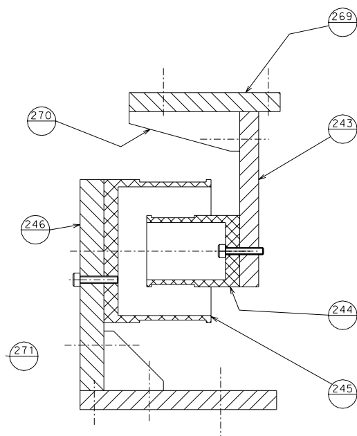
Figure 4.6: Horizontal LVDT scheme. (269) and (243) represent the supports for the secondary coil (244) hanging from the springs box. The primary coil (245) is supported by (246) to the base.
