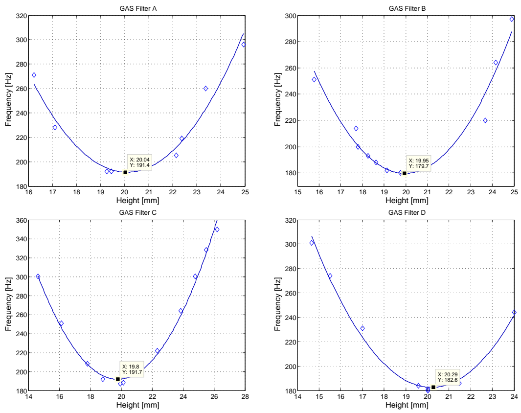
Figure 3.1: GAS filters Frequency vs Height experimental curves.
