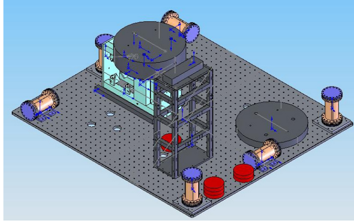
Figure 4.1: Optics table installed on HAM-SAS inside the LASTI HAM vacuum chamber.
