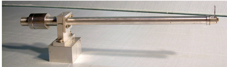
Figure 2.12: "Magic Wand" designed for HAM-SAS. At present they have not been installed in the system yet. They can provide an additional order of magnitude in vertical attenuation at 10 Hz.
