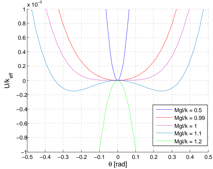
Figure 2.17: The reduced potential energy U_{pot}/\kappa is plotted for different values of the gravity elastic ratio R_{ge} = Mgl/\kappa . For R \ll 1 the system is far from instability; or R \gtrsim 1 the system becomes bi-stable; for R \gg 1 there is no stable equilibrium point and the system collapses.
