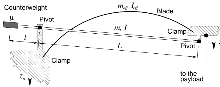
Figure 2.11: Rigid body representation of the GAS filter with a wand. For sake of simplicity just one blade and one wand are sketched. Because of its distributed mass, the low frequency blade's dynamics can be approximated with a rigid body with effective mass and moment of inertia rotating about an horizontal axis. A wand with a counterweight connected as shown in the figure, provides a way of properly tune the center of percussion and remove the transmissibility saturation.
