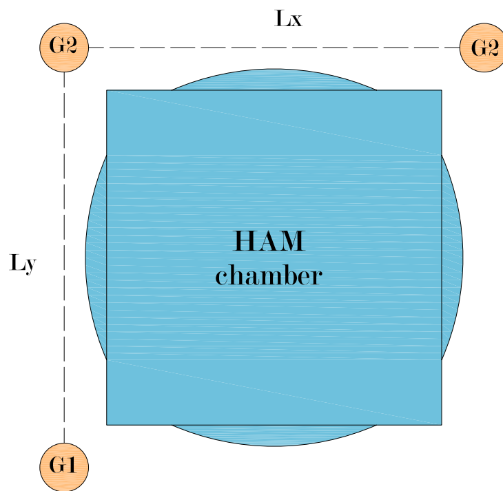
Figure 4.14: Guralp seismometers placements around the HAM chamber.
