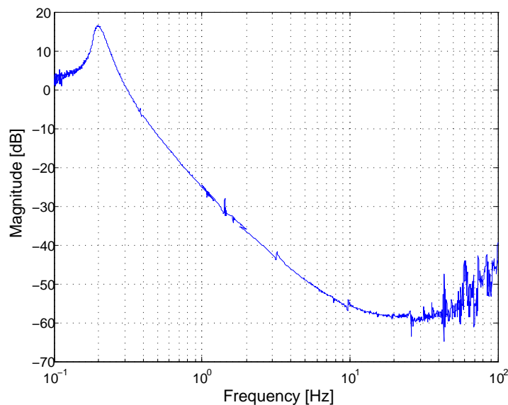
Figure 2.6: GAS filter transmissibility measured at Caltech in 2005 on a three blade, 3mm thick bench prototype [13]
