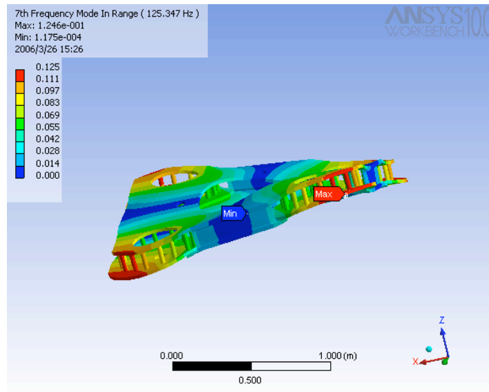
Figure 2.22: Simulations of the internal modes of the spring box brought to the introduction of later stiffeners into the structure.
