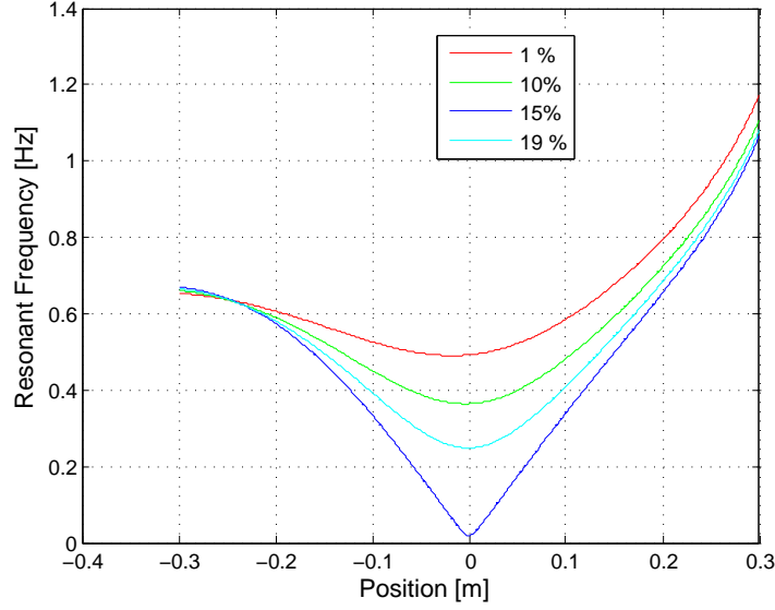
Figure 2.10: Resonant frequency to equilibrium position for several values of compression. The minimum moves from the original position.
