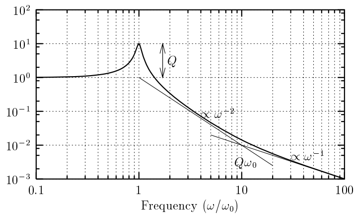
Figure 1.9: Response of a simple harmonic isolator with finite Q .
