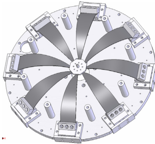
Figure 2.5: HAM-SAS GAS Filter
