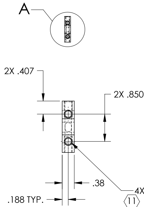
DETAIL A SCALE 2 : 3 BOTH ENDS
