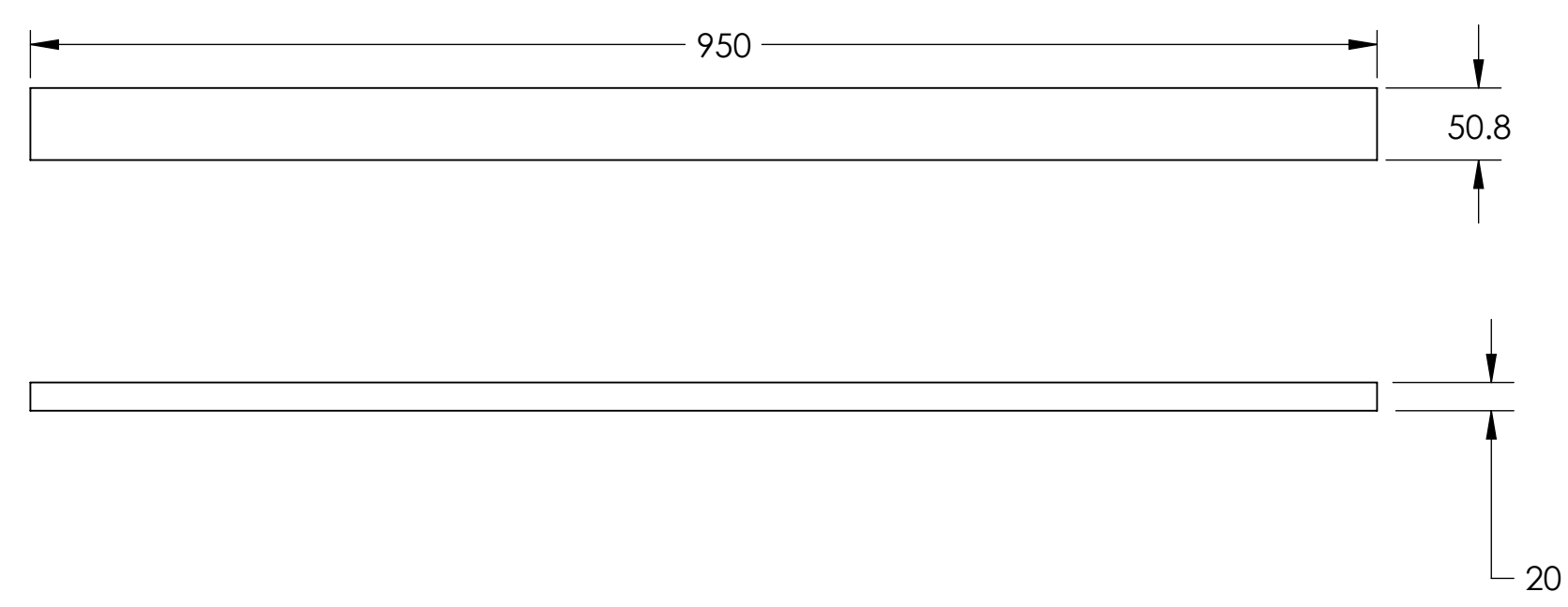
MIDDLE MATERIAL: 6061-T6 ALUM ALLOY
