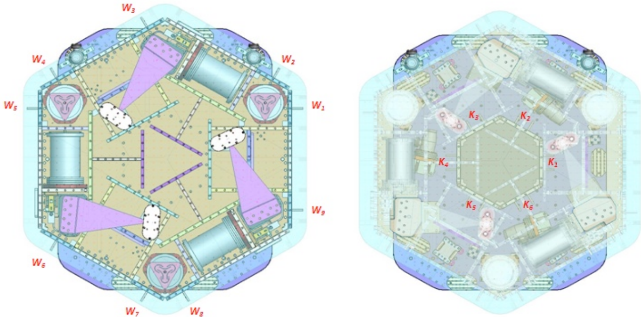
Figure 7: Keel Masses and Wall masses location
