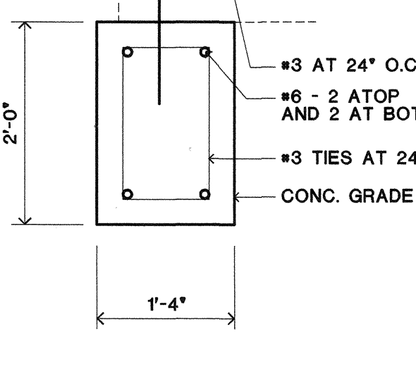
4 GRADE BEAM TYP. 3/4" - 1'-0"
