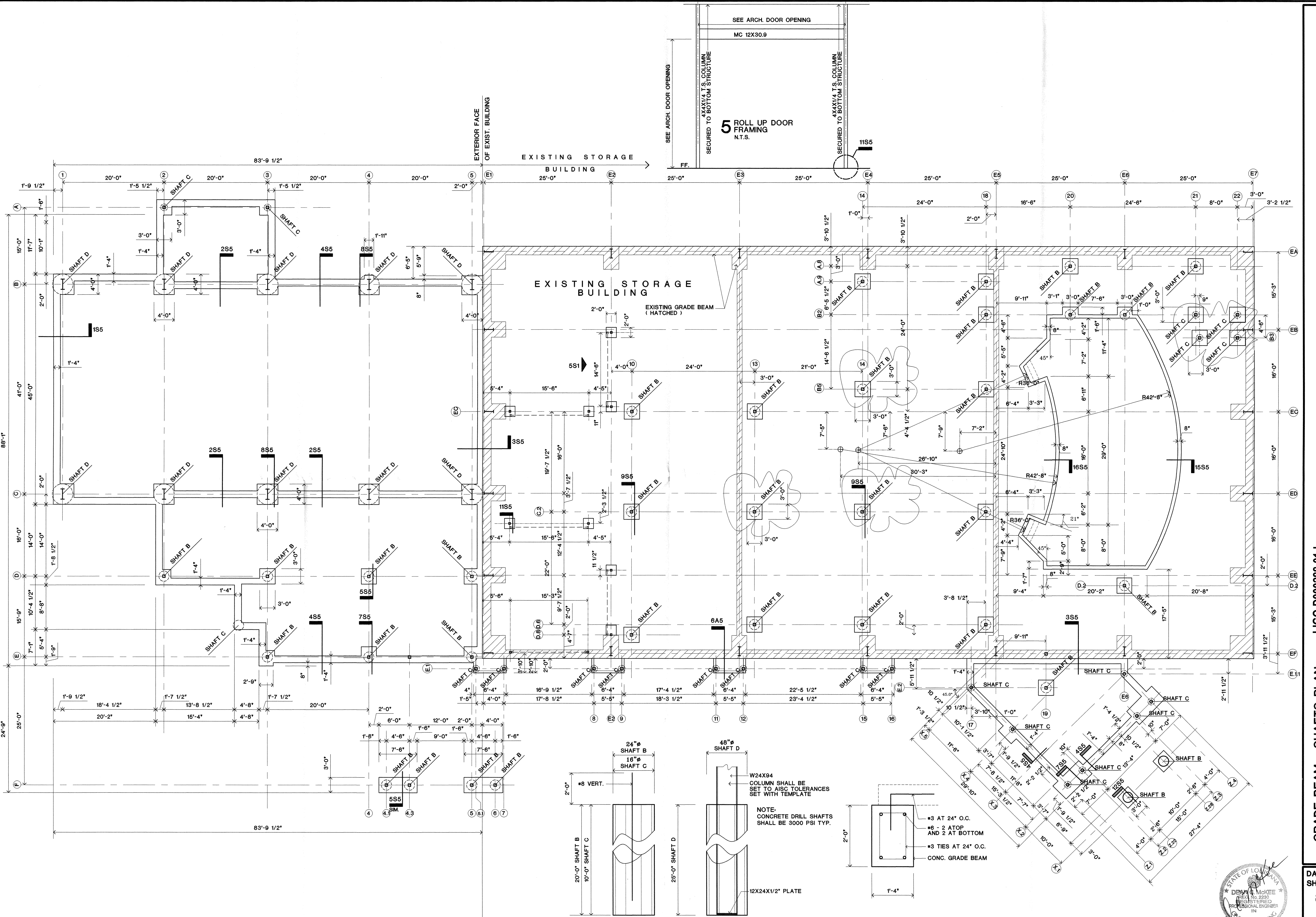
1 GRADE BEAM - DRILL SHAFTS PLAN ← NEW BUILDING → EXISTING METAL BUILDING
