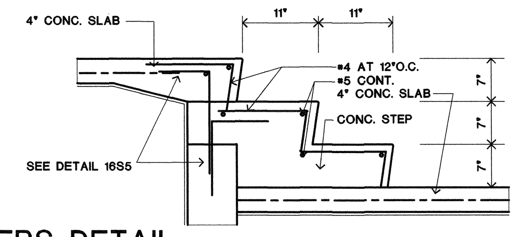
2 STEPS DETAIL 3/4" = 1'-0"
