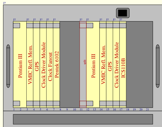
VME CRATE 2
