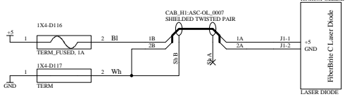
LHO 4K RCM Opt Lever Laser Diode
