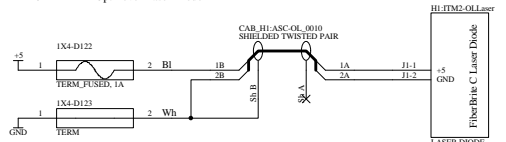
LHO 4K ITMY Opt Lever Laser Diode
