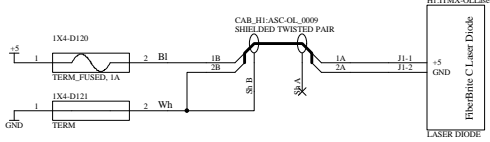
LHO 4K ITMX Opt Lever Laser Diode
