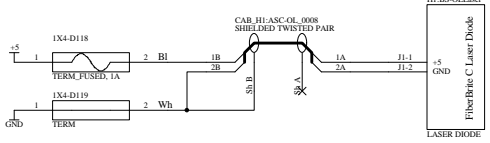
LHO 4K BS Opt Lever Laser Diode
