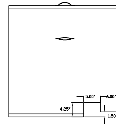
Notched Side Panel - 1 Required
