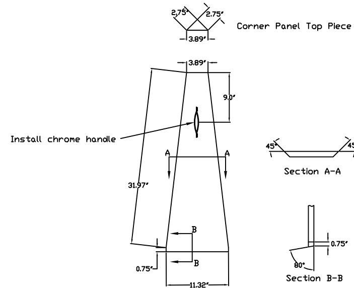
Corner Panels - 4 Required
