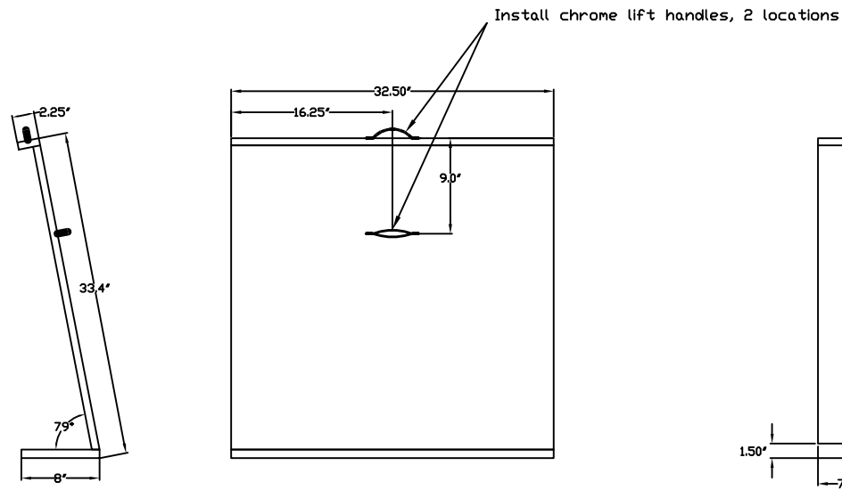
Std. Side Panels - 14 Required
