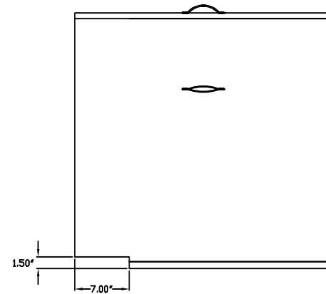
Notched Side Panel - 1 Required
