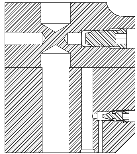
SECTION BW-BW
