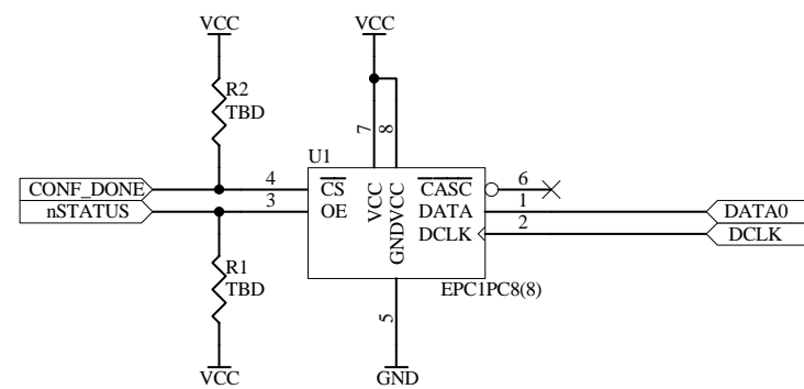
1K Pull-ups on Timing Board
