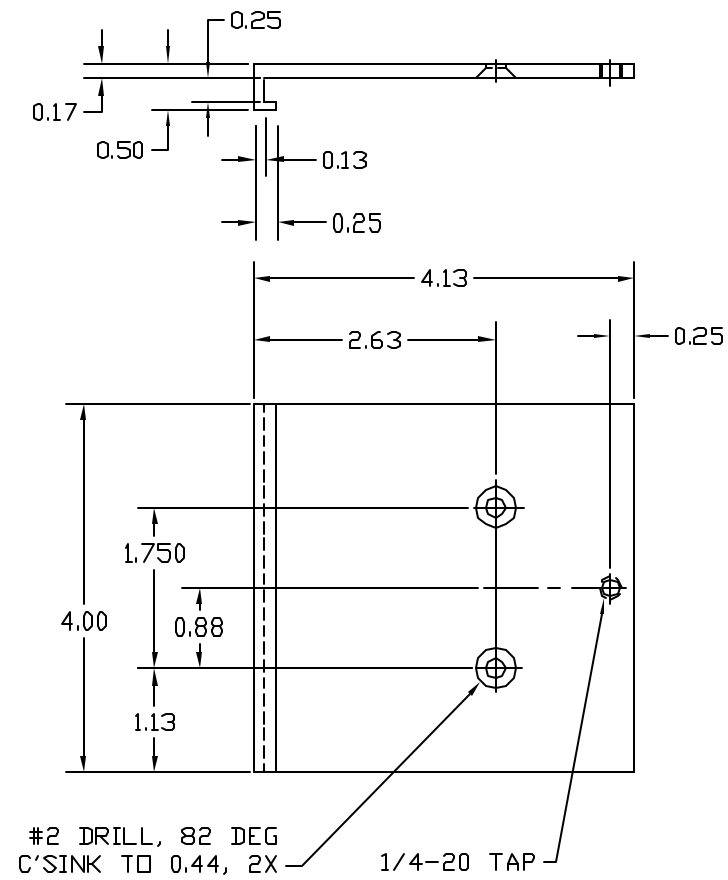
SUPPORT 3 REQ'D. MATERIAL: 6061-T6 ALUM.
