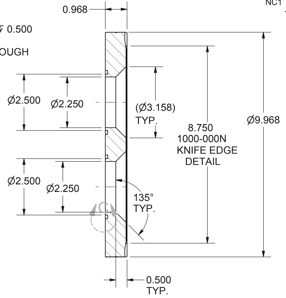
SECTION B-B SCALE 3 / 8
