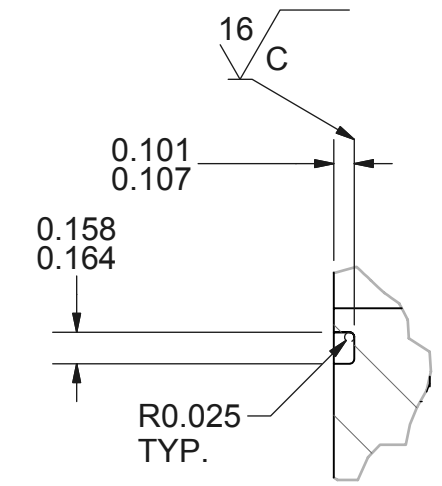
DETAIL C SCALE 1 : 1 TYP. 2X
