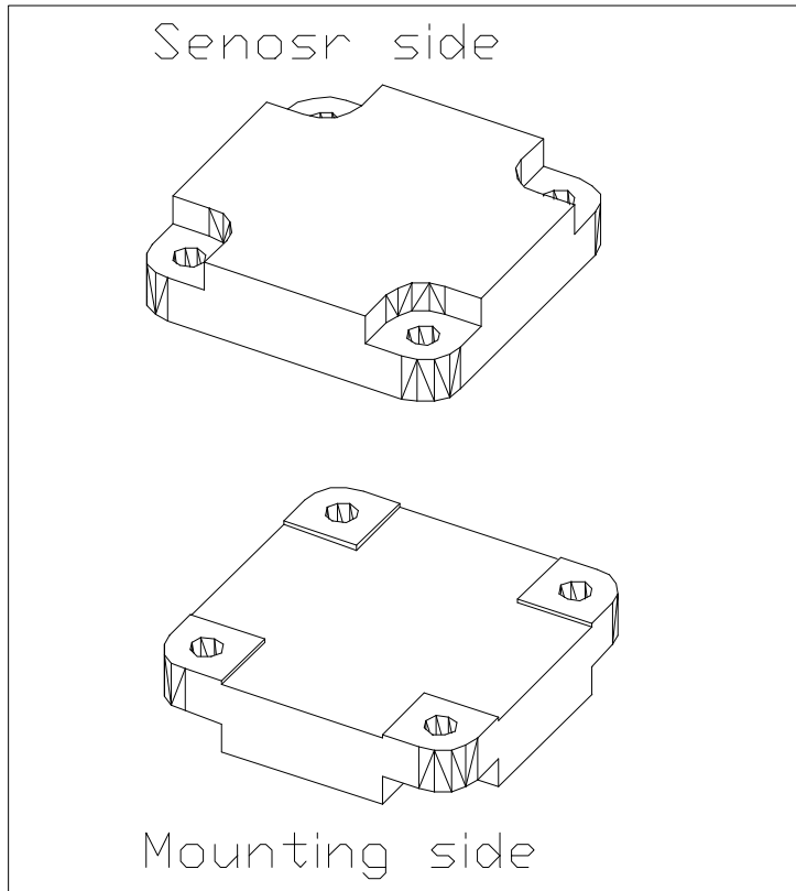
Hi-Stability 10 mm sensor ADE # 020536-A01
