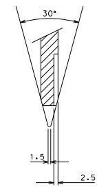
section A-A scale 1/1
