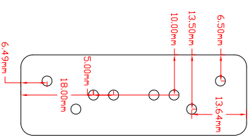
D070155-00-C DMC Graveyard Wire Loom Bottom Plate - Aluminum Top View tolerance - 0.05mm
