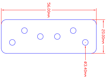
D070155-00-C DMC Wire Loom Top Plate - Aluminum Bottom View tolerance - 0.05mm
