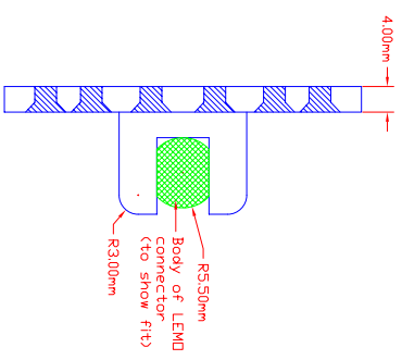
D070155-00-C DMC Graveyard Wire Loom Top Plate - Aluminum Side View tolerance - 0.05mm
