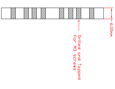
D070155-00-C DMC Graveyard Wire Loom Bottom Plate - Aluminum Side View tolerance - 0.05mm
