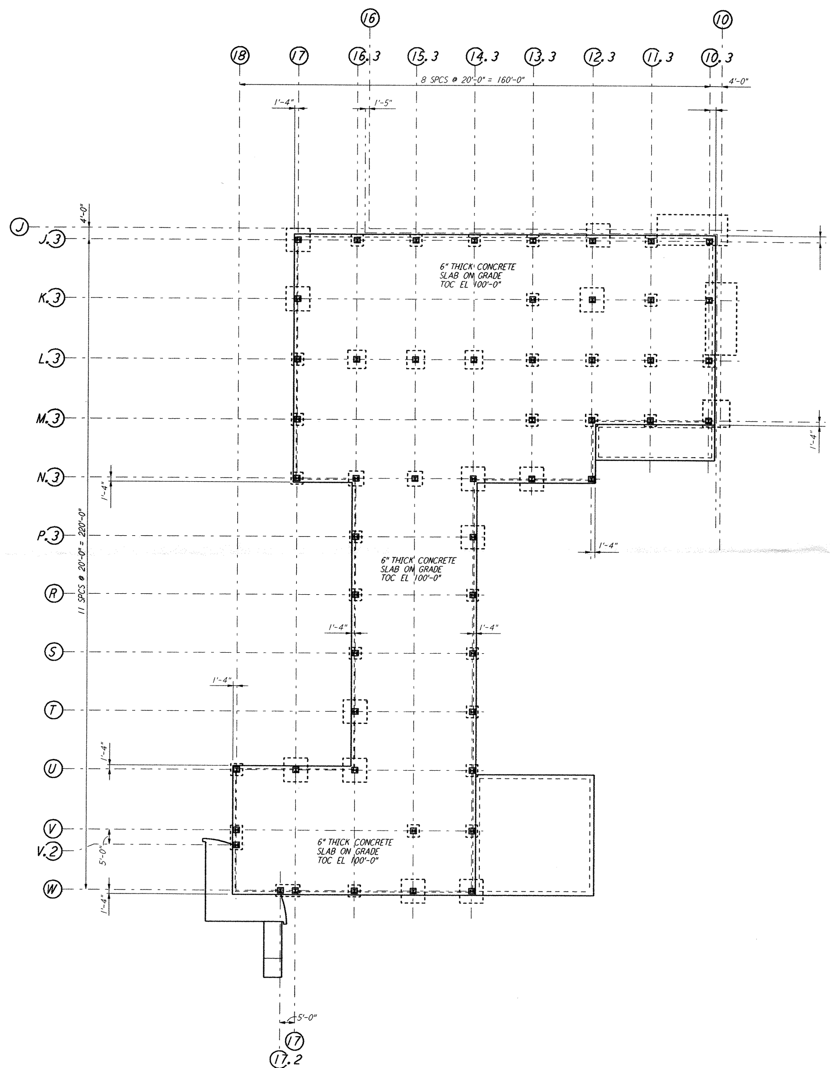
FOUNDATION PLAN 1/16" = 1'-0"
