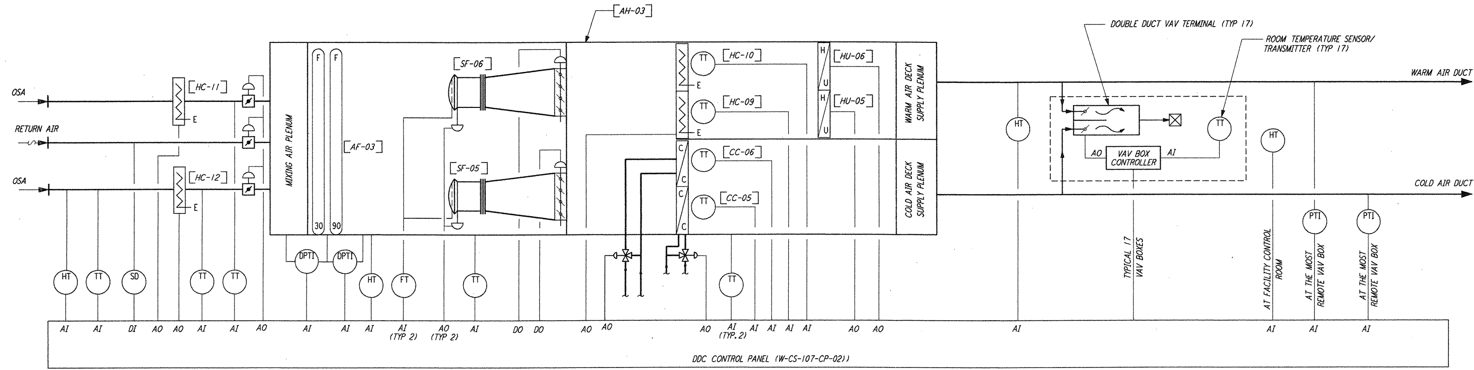
OSB AIR FLOW & CONTROL DAIGRAM (AH-03)
