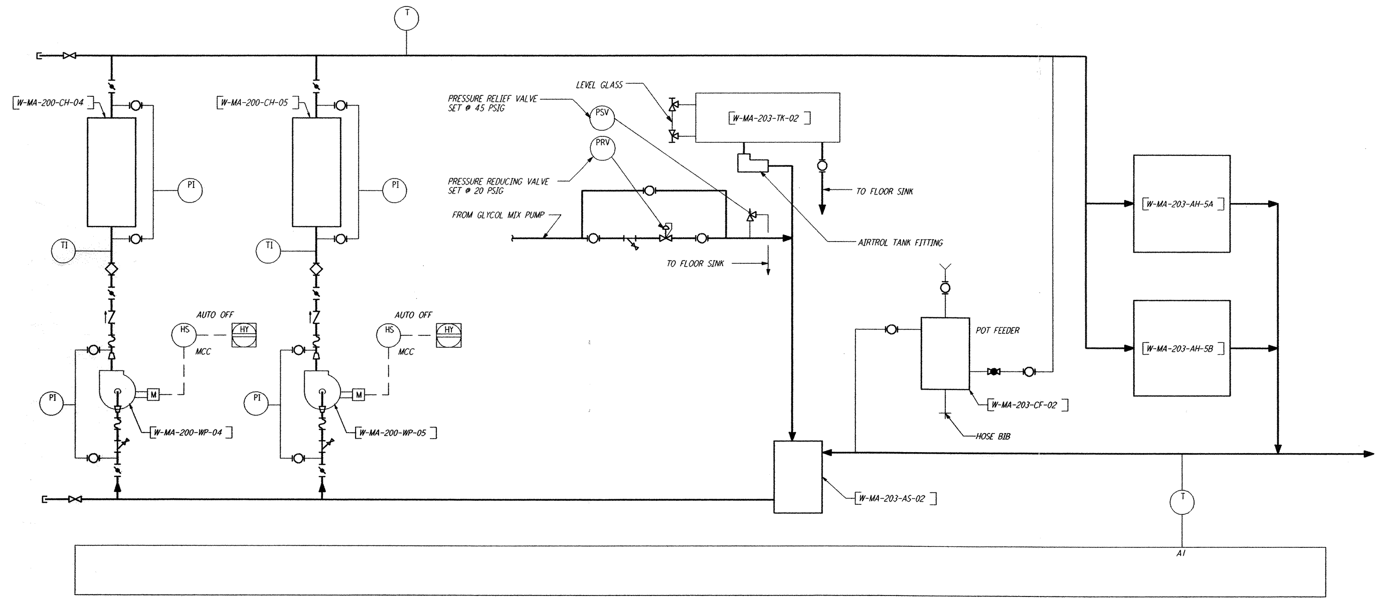
CHILLED WATER FLOW DIAGRAM AT MID STATION "A" TYPICAL FOR MID STATION "B"
