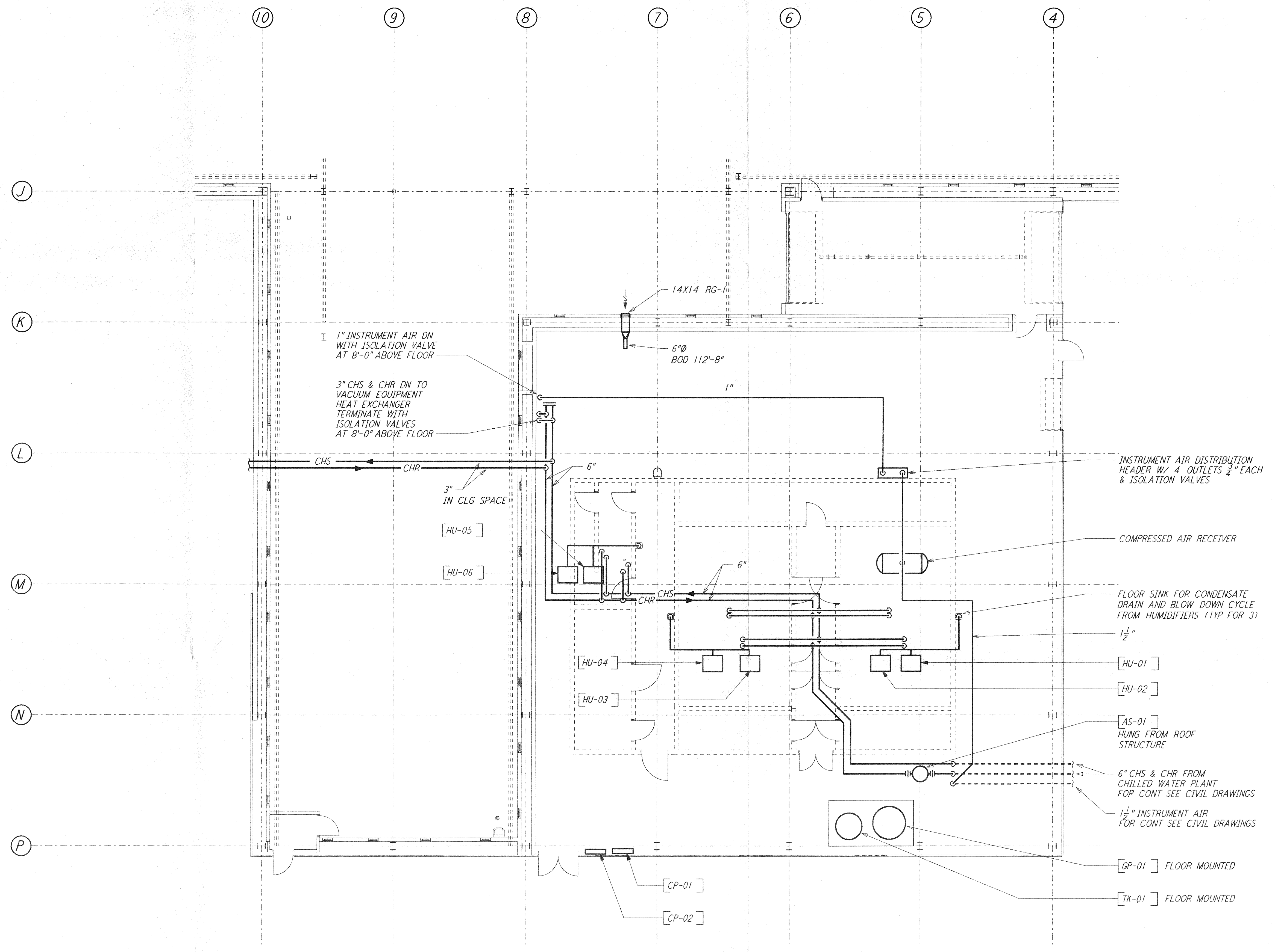
MECHANICAL ROOM PLAN \frac{1}{8}'' = 1'-0''
