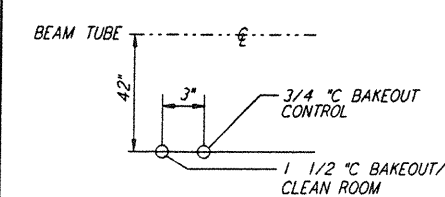
DETAIL 7 REF NTS WA-E-503 WA-E-504
