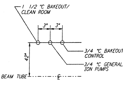
DETAIL 2 REF NTS WA-E-503 WA-E-504
