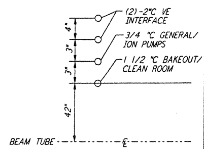
DETAIL 11 REF NTS WA-E-503 WA-E-504
