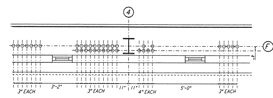
DETAIL 20 REF NTS WA-E-503
