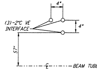
DETAIL 12 REF NTS WA-E-503 WA-E-504
