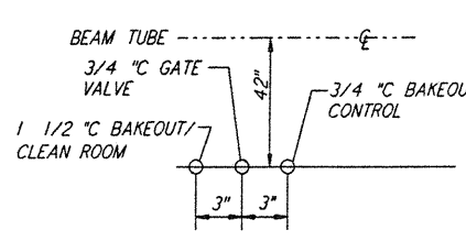
DETAIL 10 REF NTS WA-E-503
