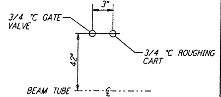
DETAIL 6 REF NTS WA-E-503
