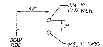
DETAIL 15 REF NTS WA-E-503
