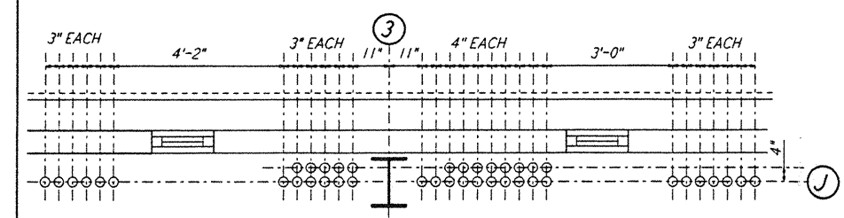
DETAIL 17 REF NTS WA-E-503
