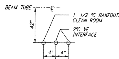
DETAIL 13 REF NTS WA-E-503 WA-E-504
