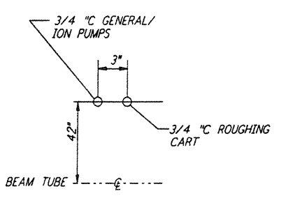
DETAIL 3 REF NTS WA-E-503 WA-E-504
