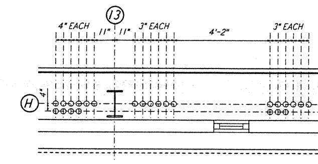
DETAIL 19 REF NTS WA-E-503
