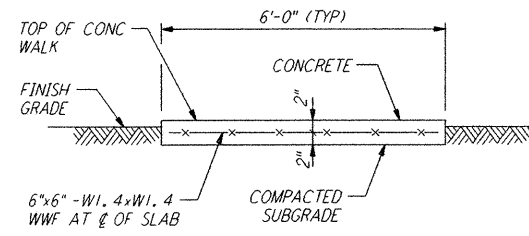
CONCRETE WALKWAY (1) NOT TO SCALE WA-C-009
