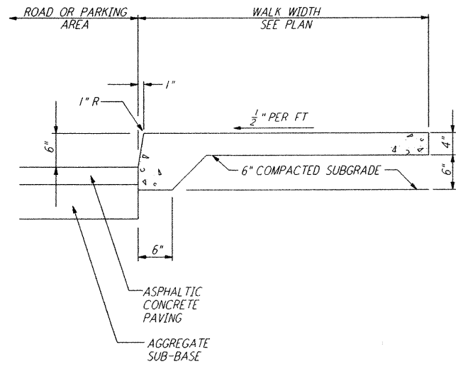
DOUBLE PURPOSE WALK (2) NOT TO SCALE WA-C-009
