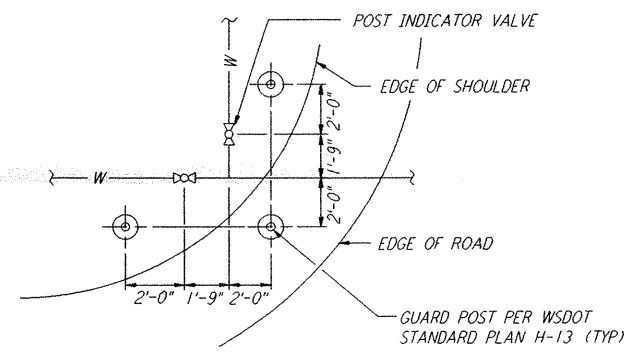
GUARD POST LOCATIONS (4) (POST INDICATOR VALVE) NOT TO SCALE WA-C-009
