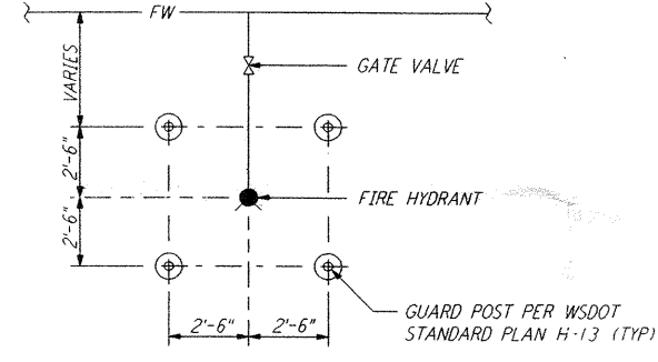
GUARD POST LOCATIONS (5) (FIRE HYDRANT) NOT TO SCALE WA-C-009
