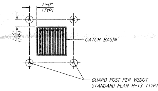
GUARD POST LOCATIONS (3) CATCH BASIN NOT TO SCALE WA-C-009
