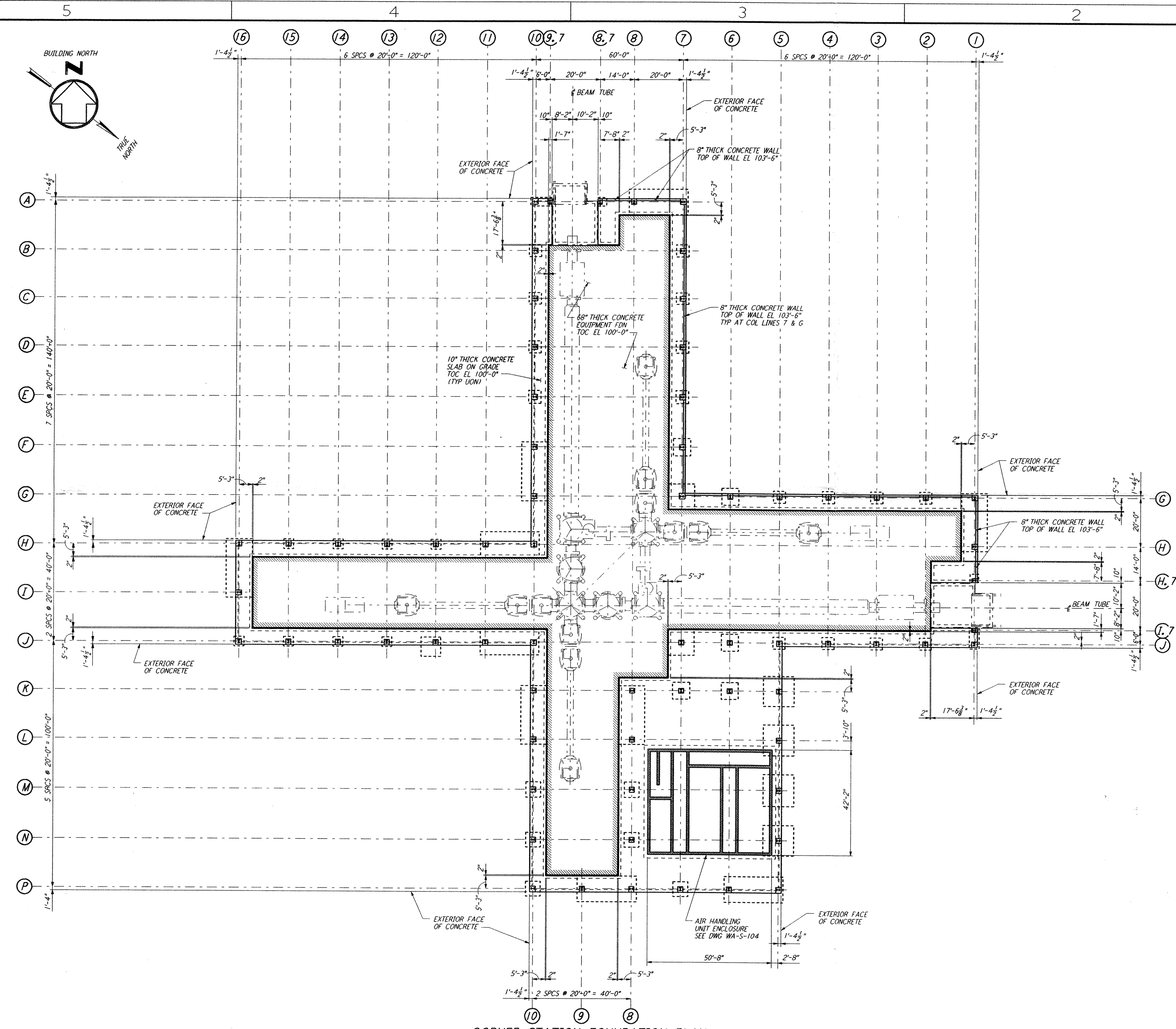
CORNER STATION FOUNDATION PLAN 1/8" = 1'-0"
