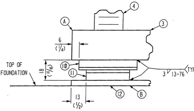
VIEW B-B
