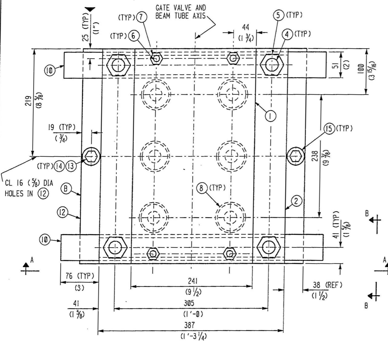
PLAN VIEW
