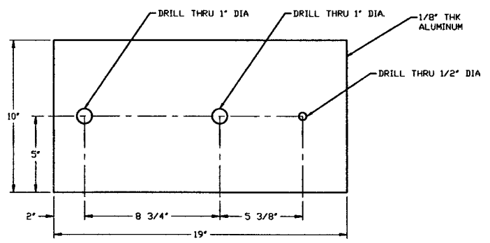
DETAIL 1
