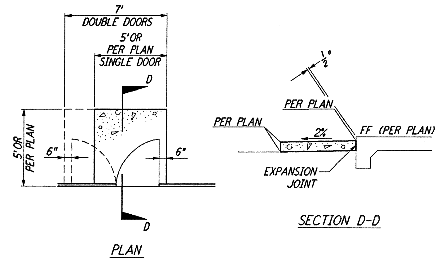
CONCRETE STOOP (1) NOT TO SCALE REF: BT-C-041, BT-C-045
