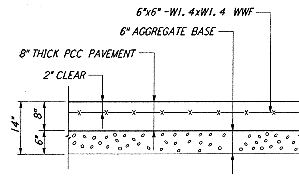
CONCRETE PAVEMENT (2) NOT TO SCALE REF: BT-C-041, BT-C-045
