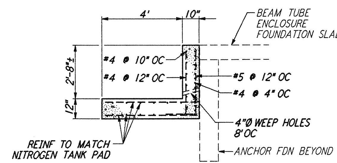
SECTION E-E
