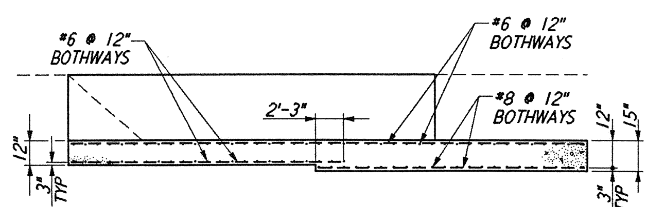
SECTION C-C
