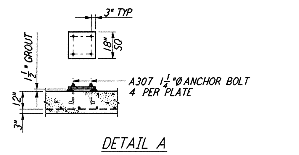
DETAIL A
