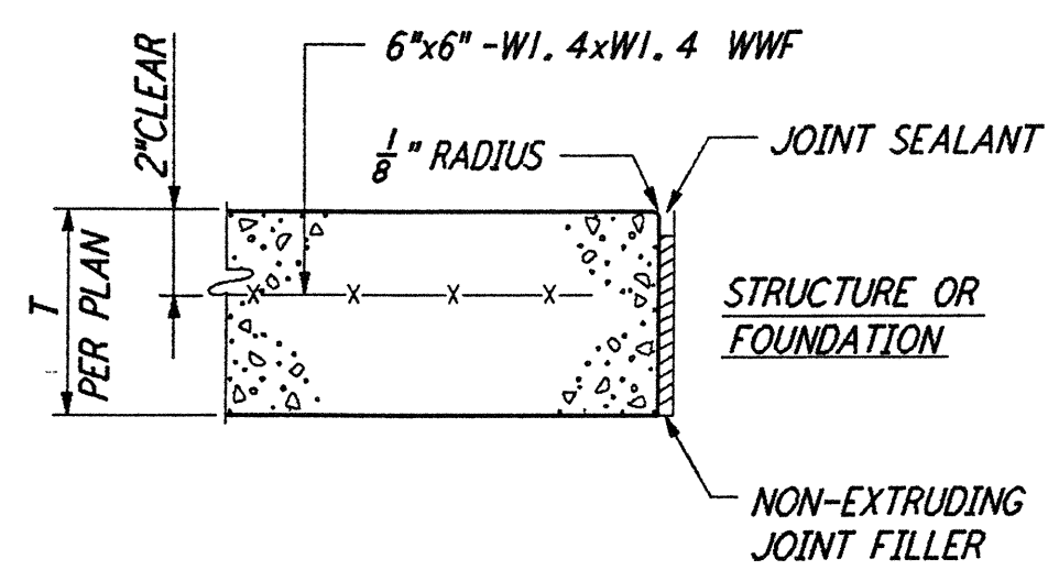
EXPANSION JOINT (3) (EJ) NOT TO SCALE REF: BT-C-041, BT-C-045
