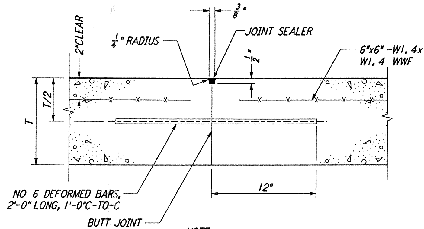
CONSTRUCTION JOINT (4) (CJ) NOT TO SCALE REF: BT-C-041, BT-C-045 (SEPARATE POURS OR END OF DAY)
