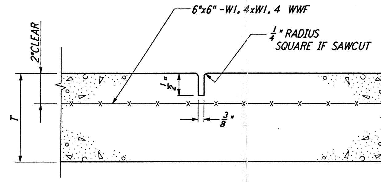
CONTRACTION JOINT (5) (CO) NOT TO SCALE REF: BT-C-041, BT-C-045 (SPACING: 20'MAX)
