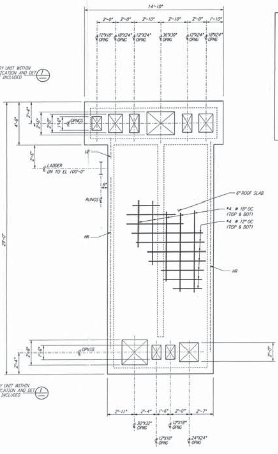
AIR HANDLING UNIT STRUCTURE CONCRETE ROOF SLAB PLAN 1/2" = 1'-0" NOT INCLUDED IN THIS CONTRACT
