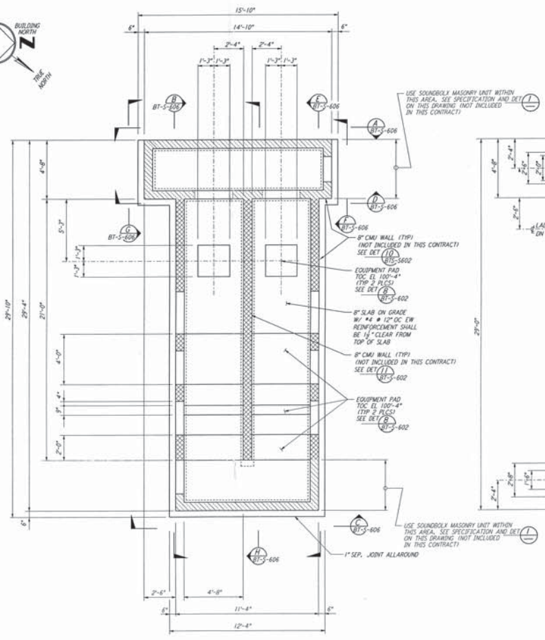
AIR HANDLING UNIT STRUCTURE FOUNDATION PLAN 1/2" = 1'-0"
