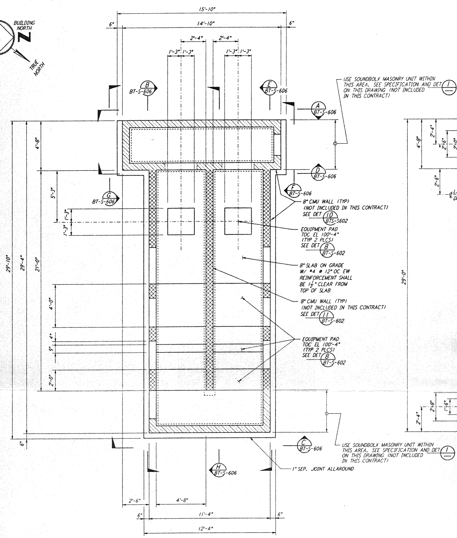
AIR HANDLING UNIT STRUCTURE FOUNDATION PLAN 1/8" = 1'-0"
