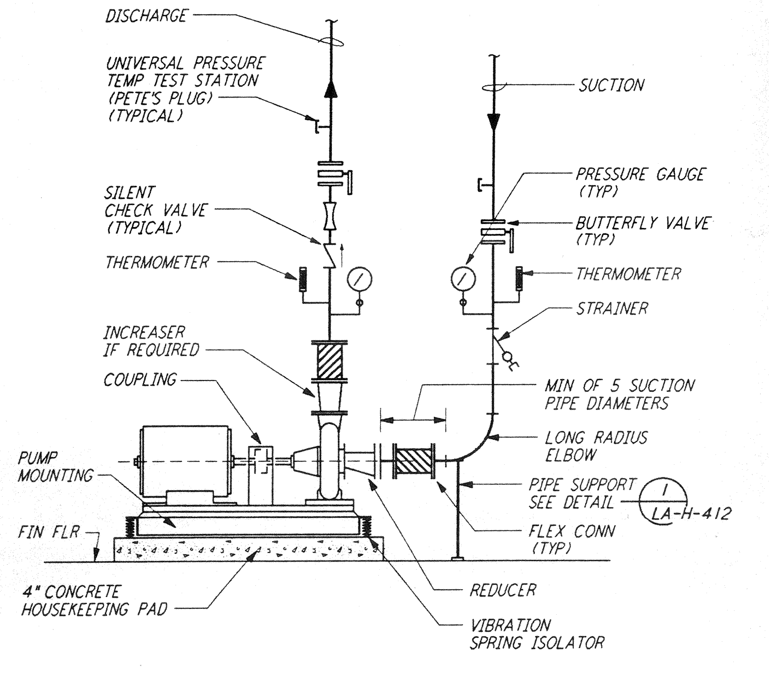
PUMP CONNECTION DETAIL (5) REF NTS LA-H-411
