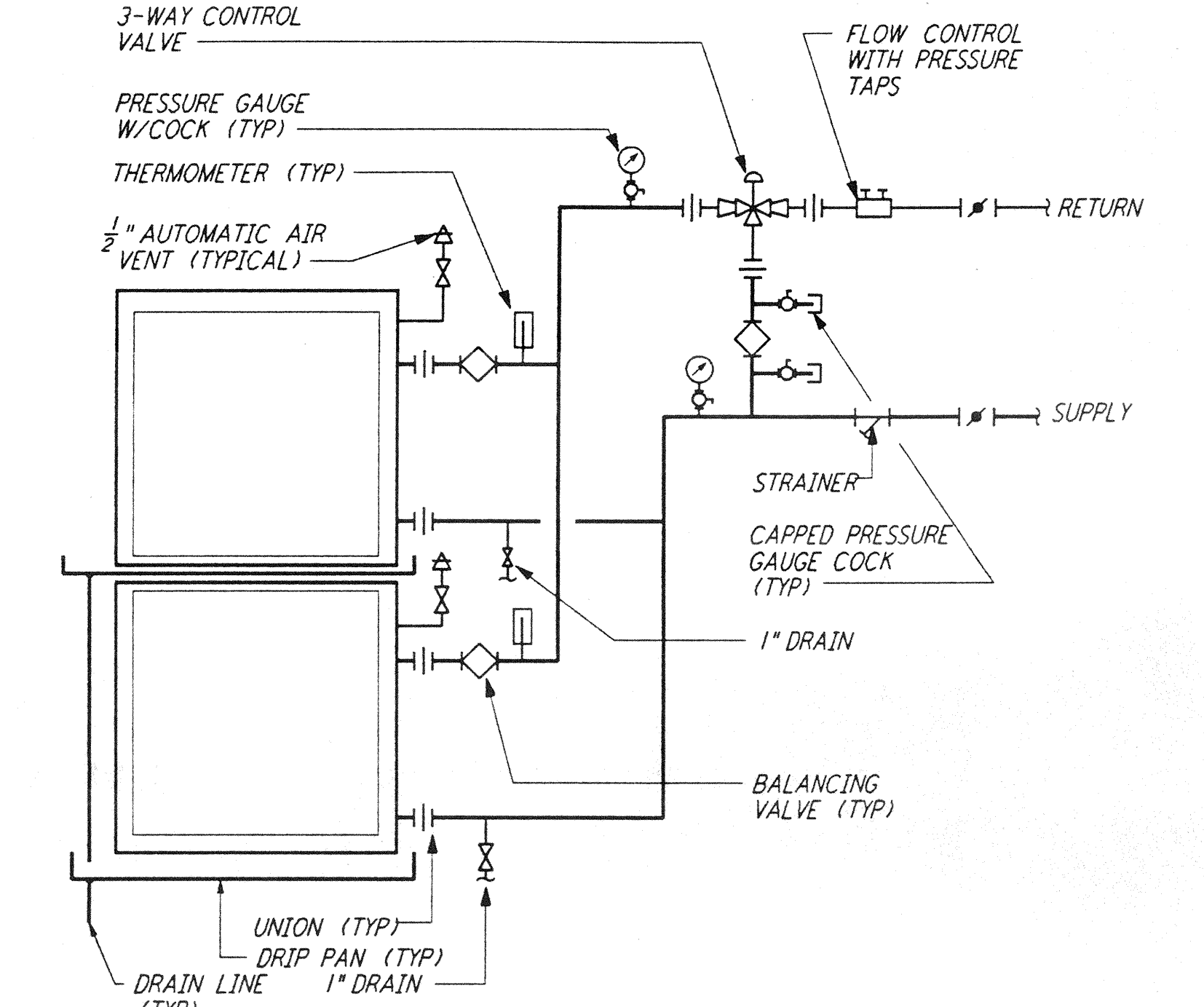
MULTIPLE COIL PIPING DETAIL (6) REF NTS LA-H-411
