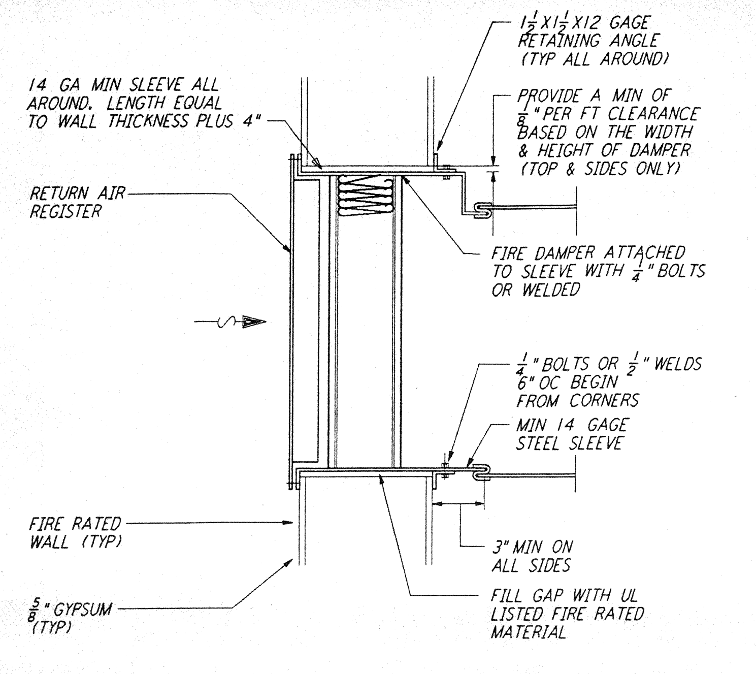
WALL MOUNTED FIRE DAMPER (1) REF NTS LA-H-411
