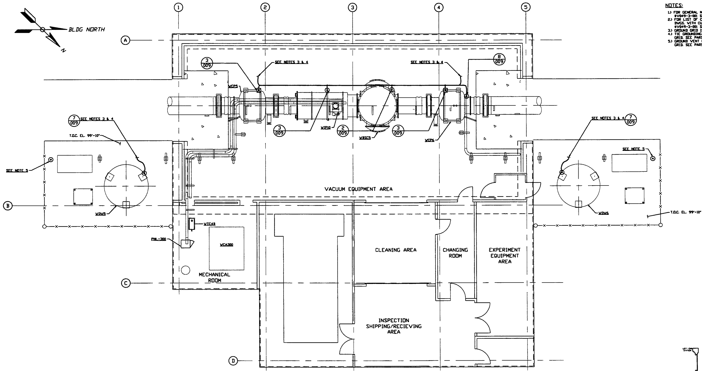
RIGHT MID STATION PLAN @ EL. 100'-0"
