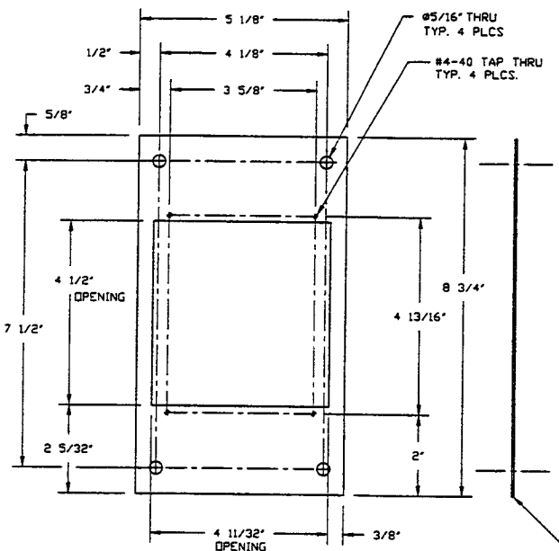
DETAIL "3" V0494107P3 SCALE HALF
