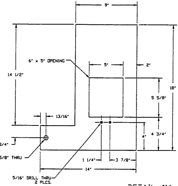
DETAIL "1" V0494107P1 SCALE 3"=1'-0"
