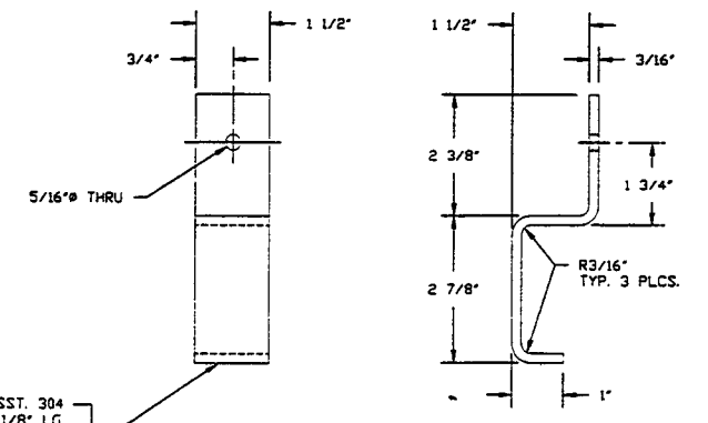
DETAIL "5" V0494107P5 SCALE HALF
