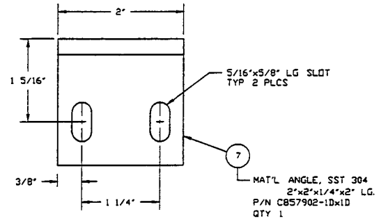
DETAIL "7" SCALE FULL
