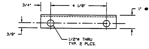
DETAIL "3" V0494107P3 SCALE HALF
