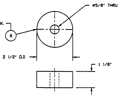
DETAIL "8" V049-4-107P8 SCALE HALF
