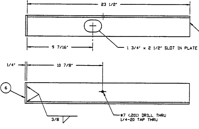
DETAIL "4" SCALE 3"=1'-0"
