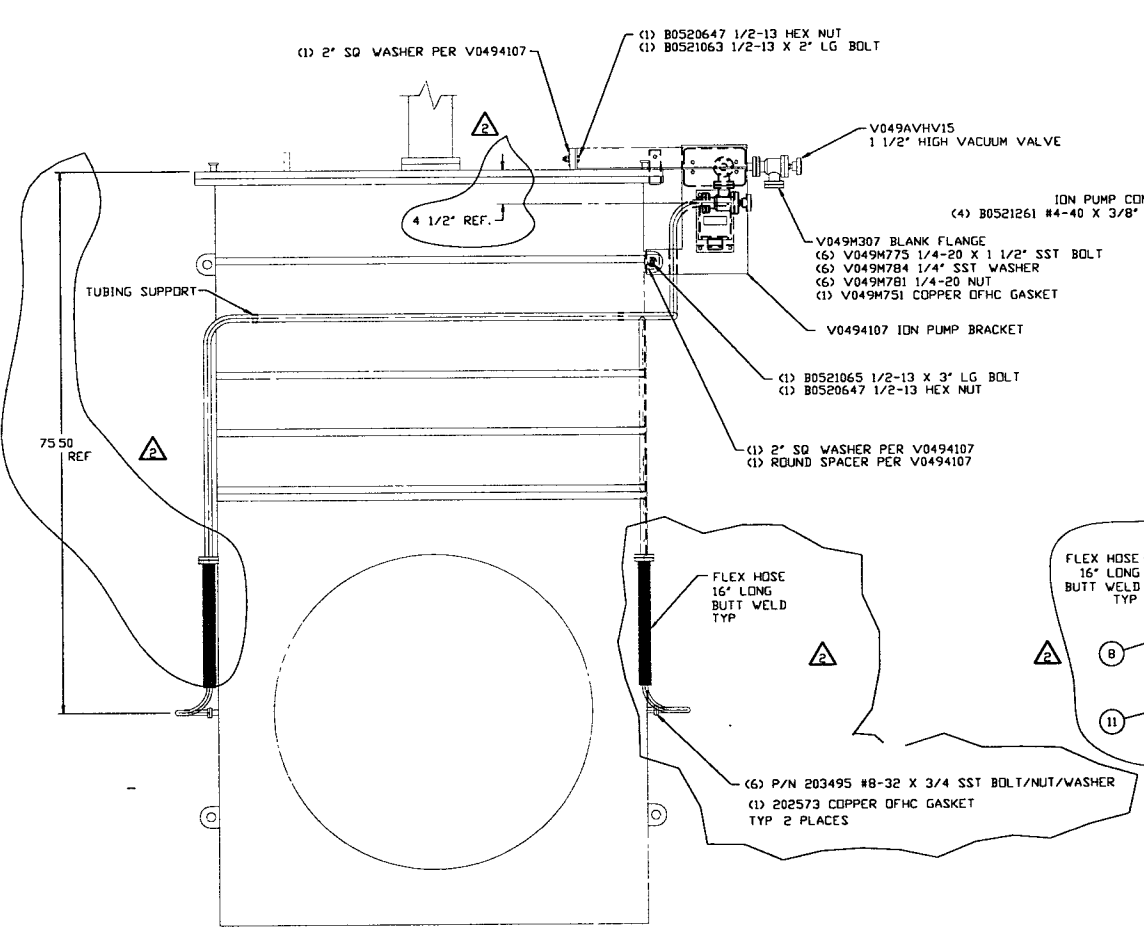
ANNULUS TUBING & ION PUMP ASSEMBLY
