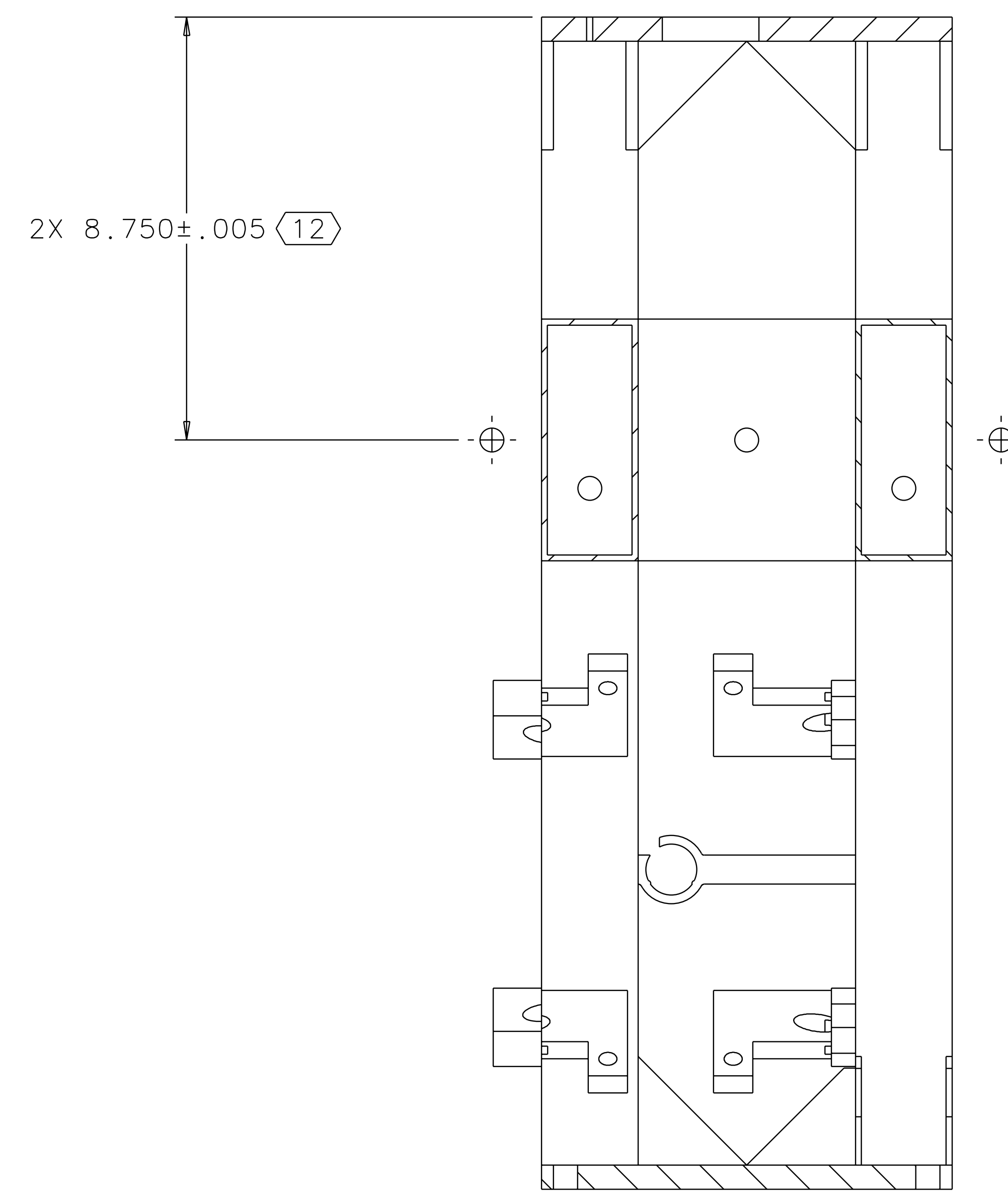
SECTION M-M (4)
