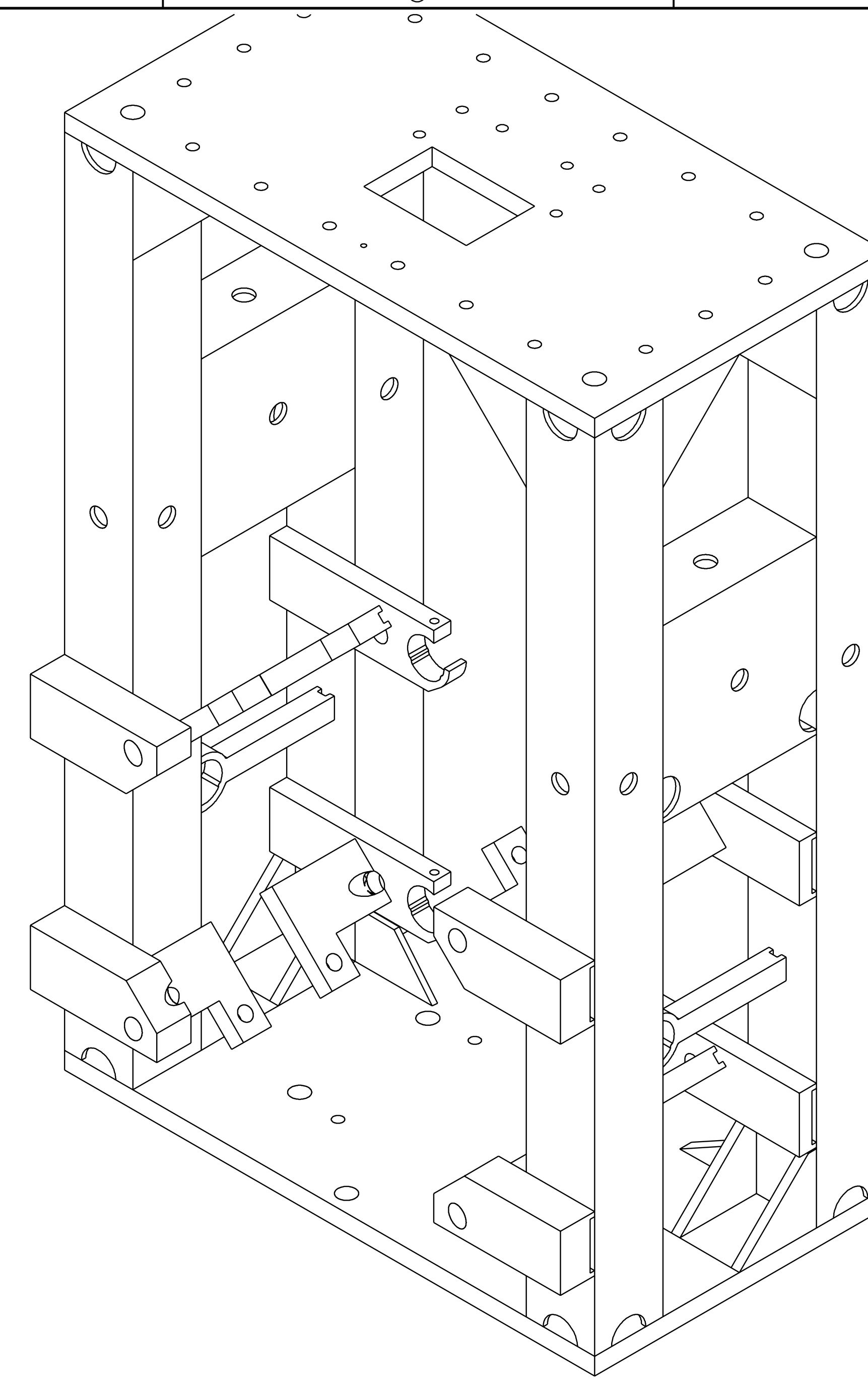
(ITEM 4 STIFFENERS REMOVED FOR CLARITY)
