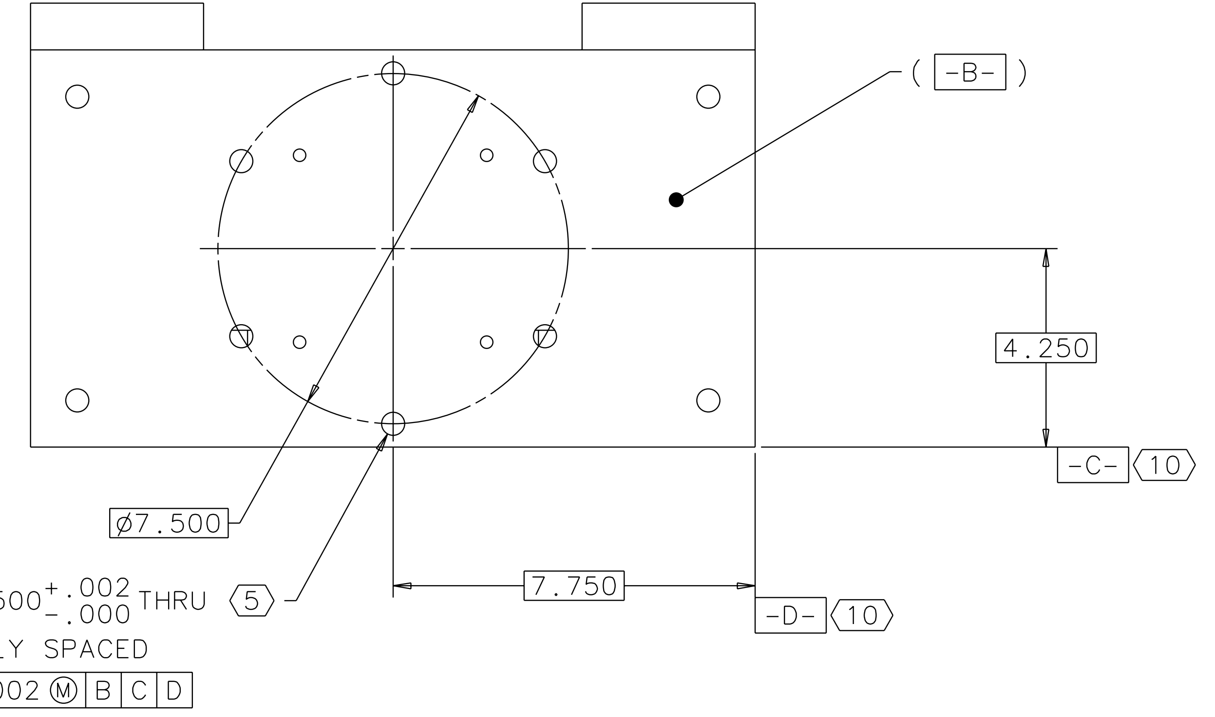
VIEW C-C 1
